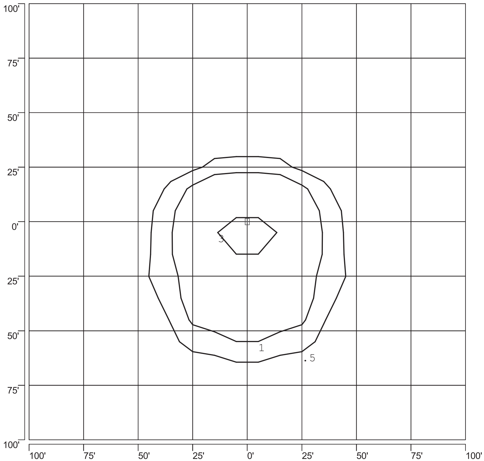
ISOFOOTCANDLE PLOT: VBMAG1B_2-PS 250W PSMH TYPE IV 25' AFG - 0 DEGREE TILT
