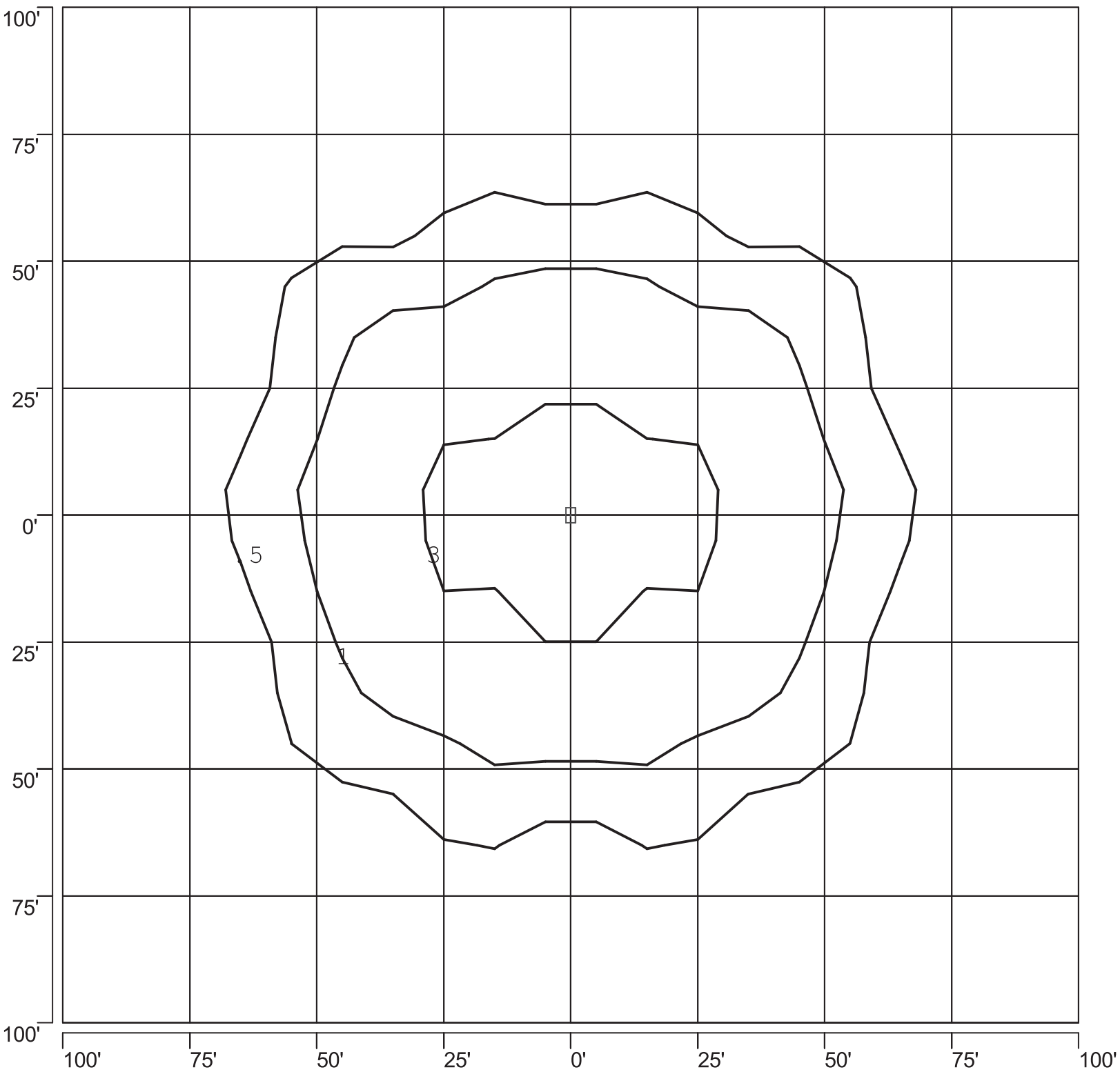
ISOFOOTCANDLE PLOT: VBMAF3B_1-PS 400W PSMH TYPE V 25' AFG - 0 DEGREE TILT
