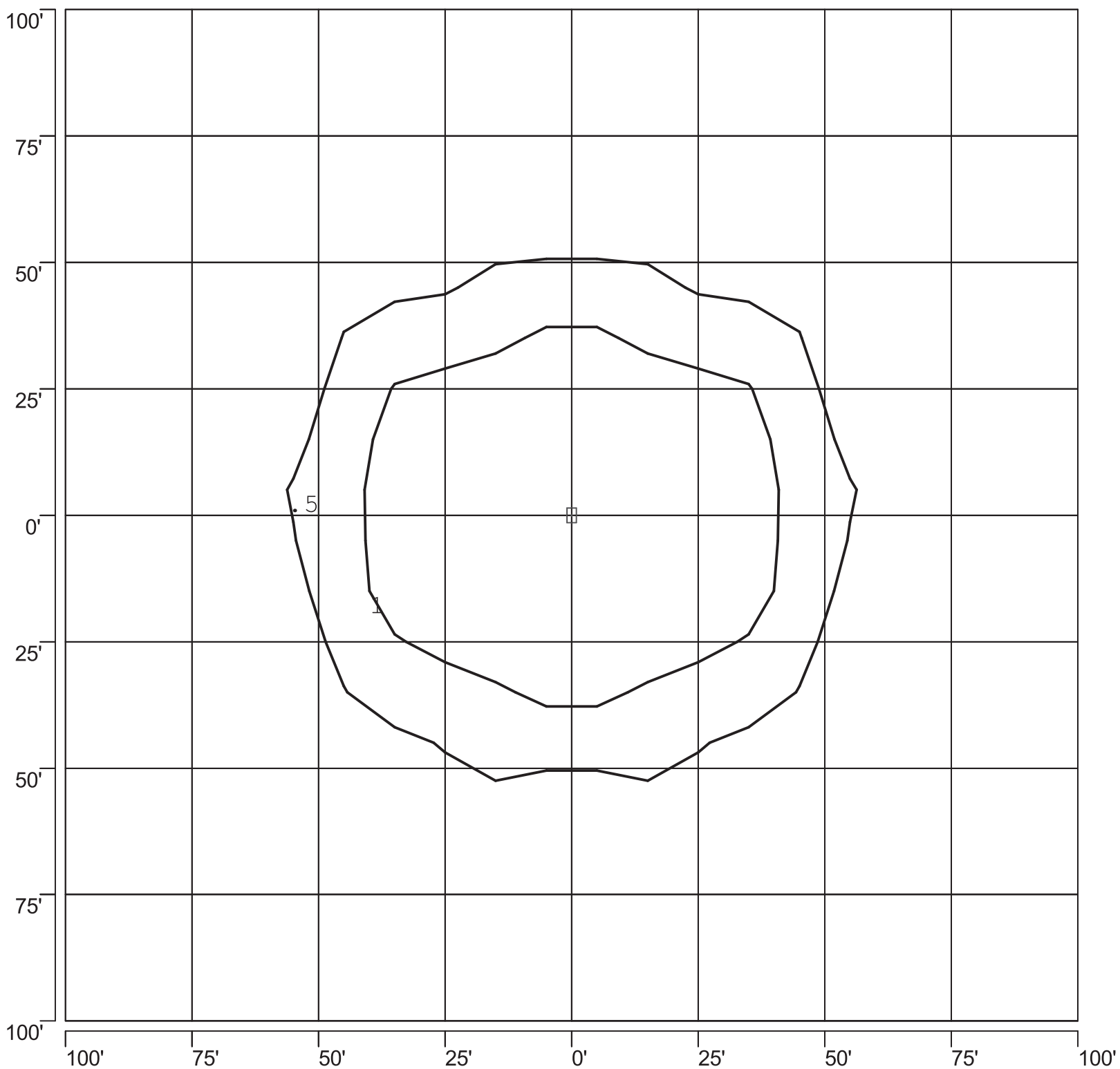
ISOFOOTCANDLE PLOT: VBMAF1B_1-PS 250W PSMH TYPE V 25' AFG - 0 DEGREE TILT
