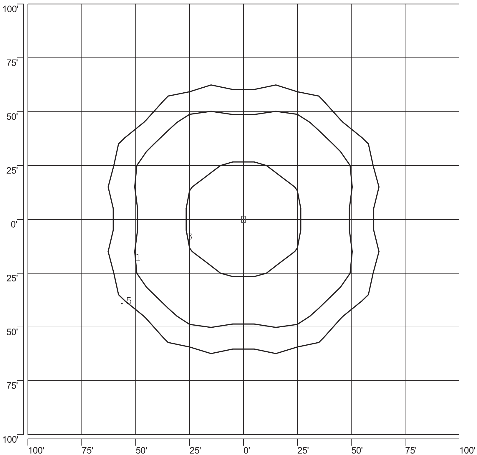
ISOFOOTCANDLE PLOT: VBMAE3B_2-PS 400W PSMH TYPE V 25' AFG - 0 DEGREE TILT
