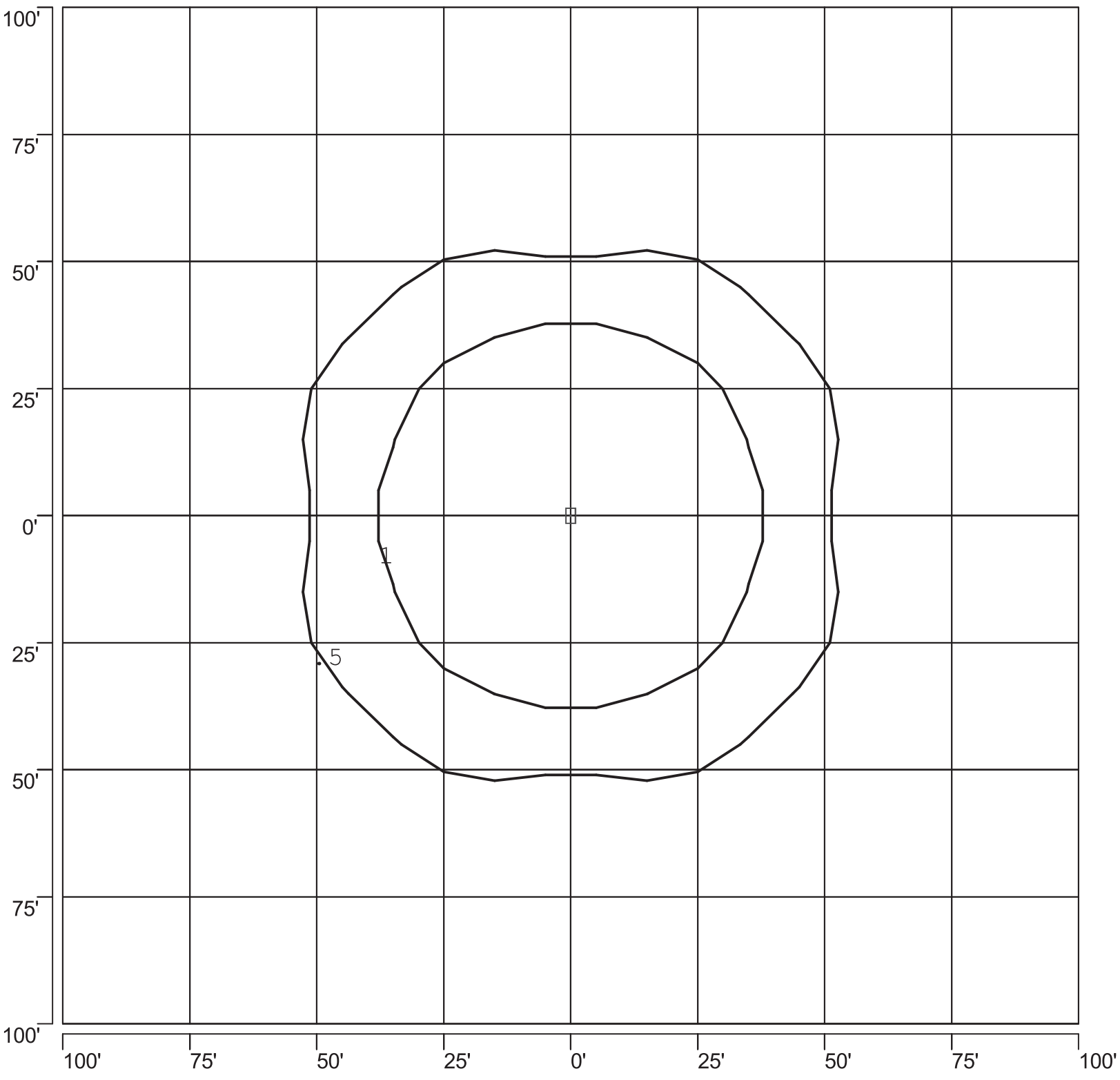
ISOFOOTCANDLE PLOT: VBMAE1B_2-PS 250W PSMH TYPE V 25' AFG - 0 DEGREE TILT
