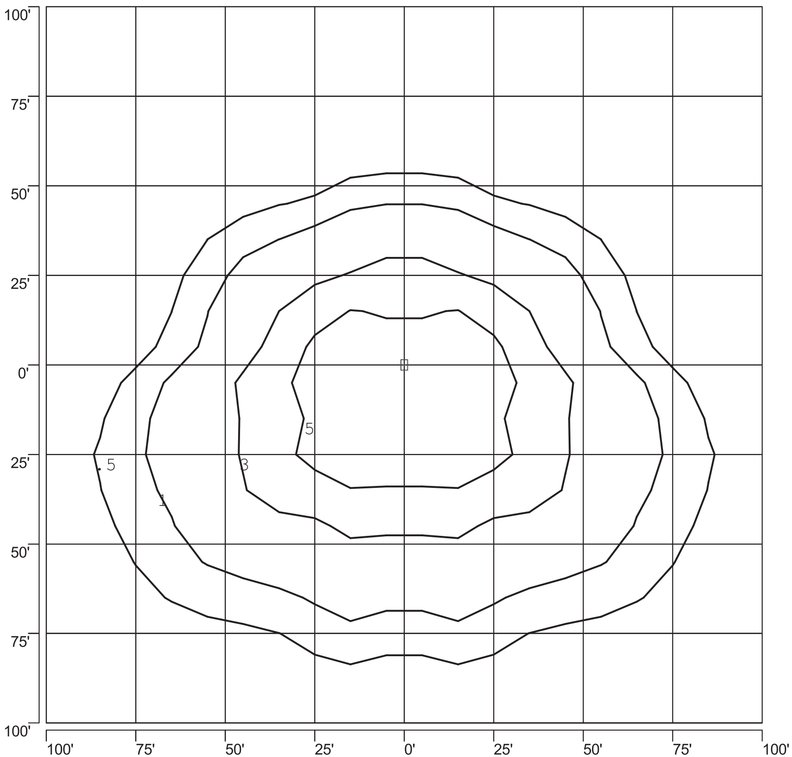
ISOFOOTCANDLE PLOT: VBLAL6B_2-PS 750W PSMH TYPE III 30' AFG - 0 DEGREE TILT
