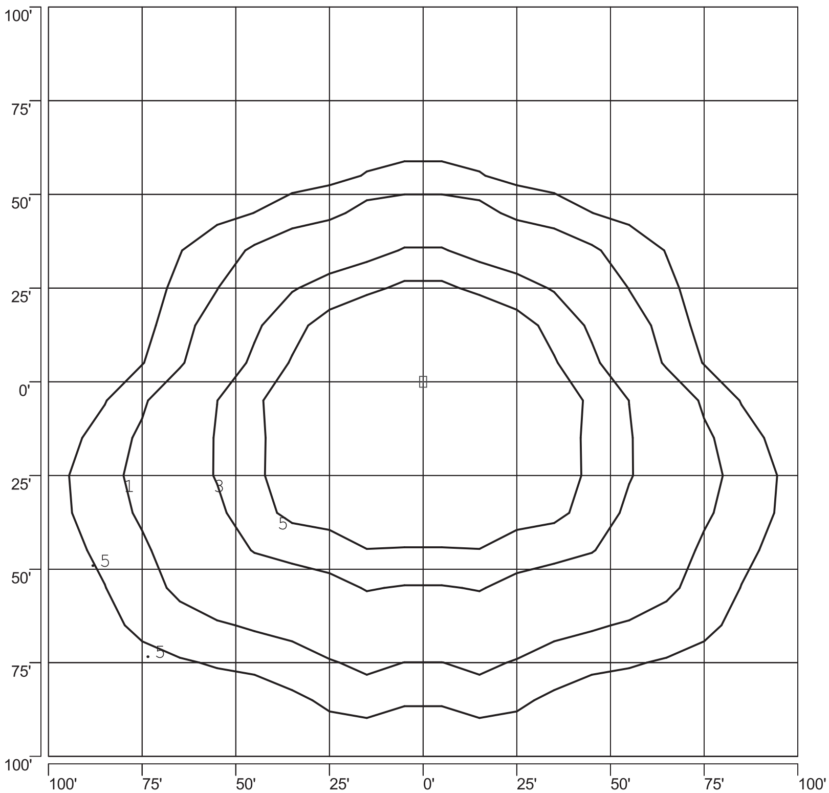
ISOFOOTCANDLE PLOT: VBLAL1B_2 1000W MH TYPE III 30' AFG - 0 DEGREE TILT
