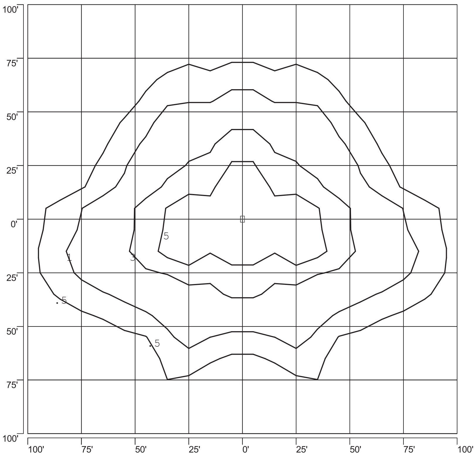
ISOFOOTCANDLE PLOT: VBLAK6B_2-PS 750W PSMH TYPE II 30' AFG - 0 DEGREE TILT
