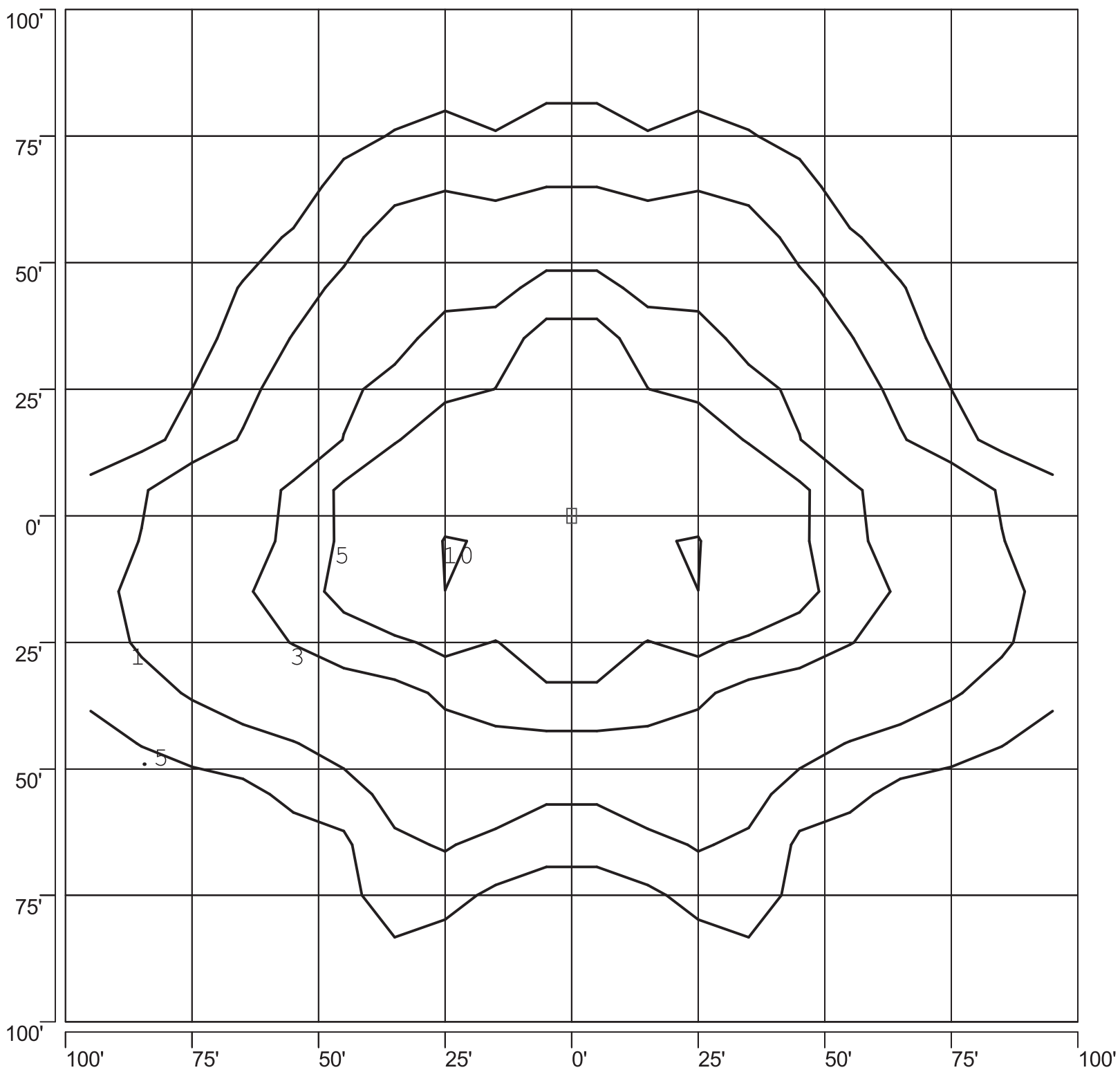
ISOFOOTCANDLE PLOT: VBLAK1B_2 1000W MH TYPE II 30' AFG - 0 DEGREE TILT
