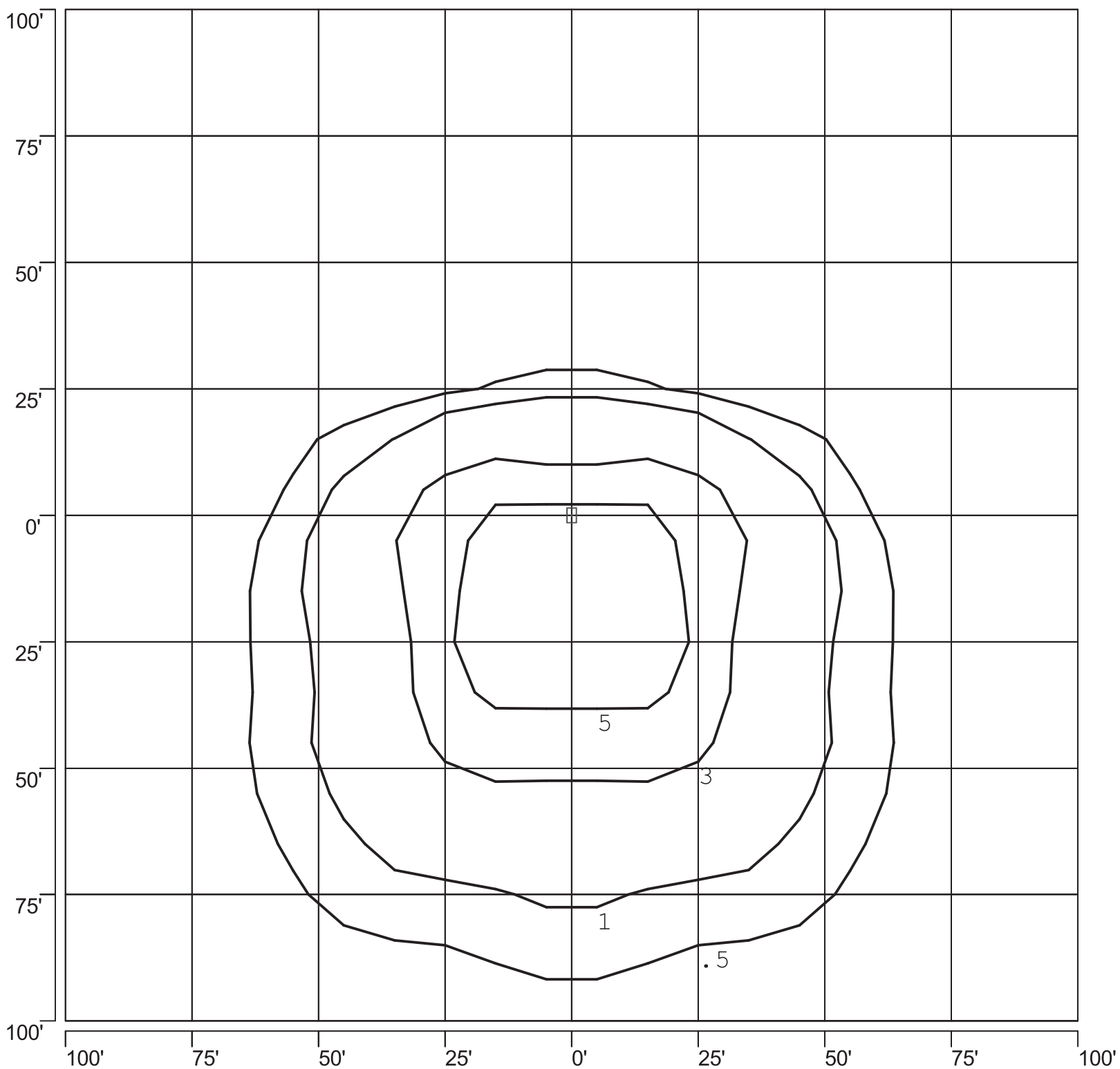
ISOFOOTCANDLE PLOT: VBLAH6B_2-PS 750W PSMH TYPE IV 30' AFG - 0 DEGREE TILT
