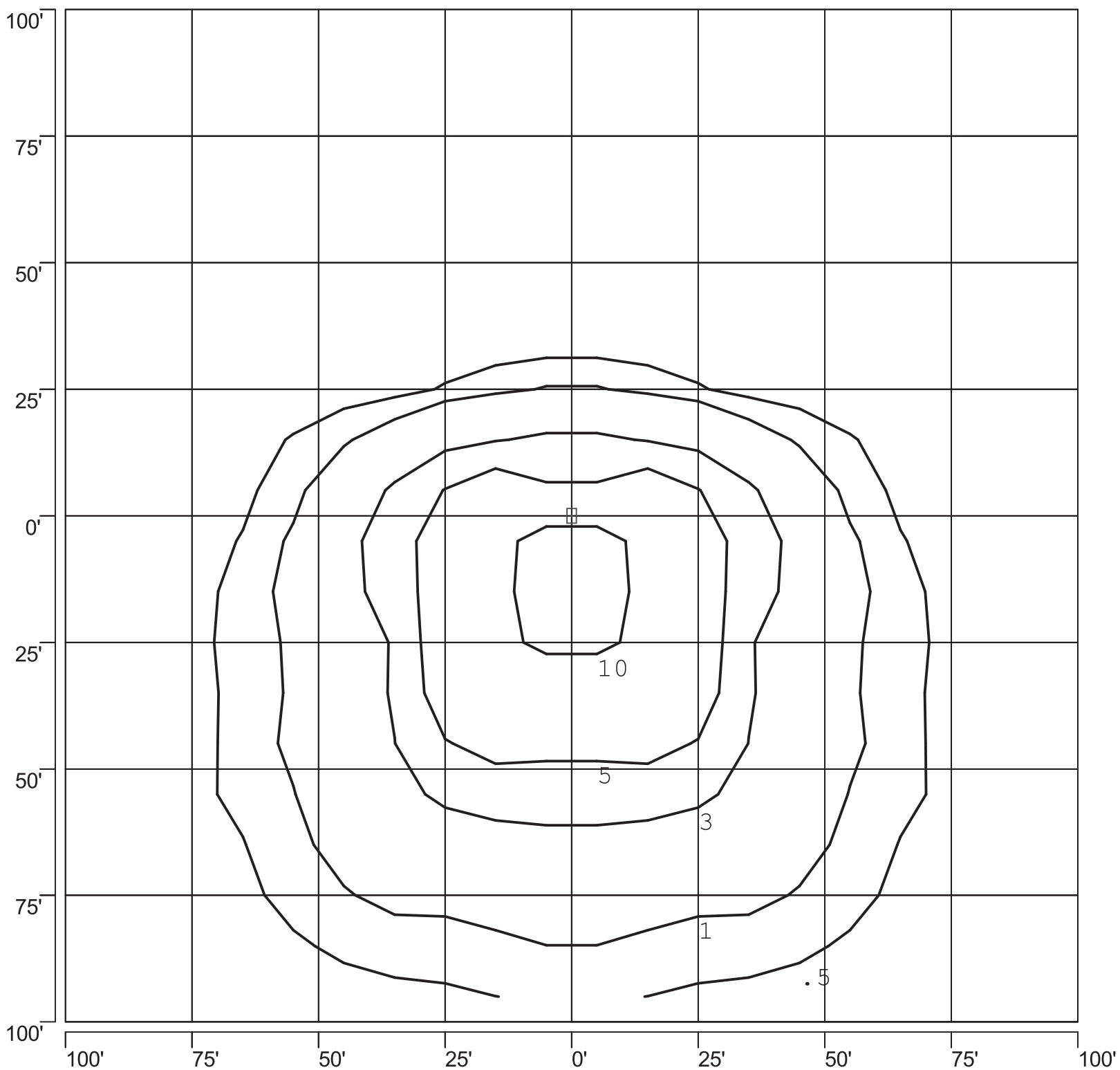
ISOFOOTCANDLE PLOT: VBLAH1B_2 1000W MH TYPE IV 30' AFG - 0 DEGREE TILT
