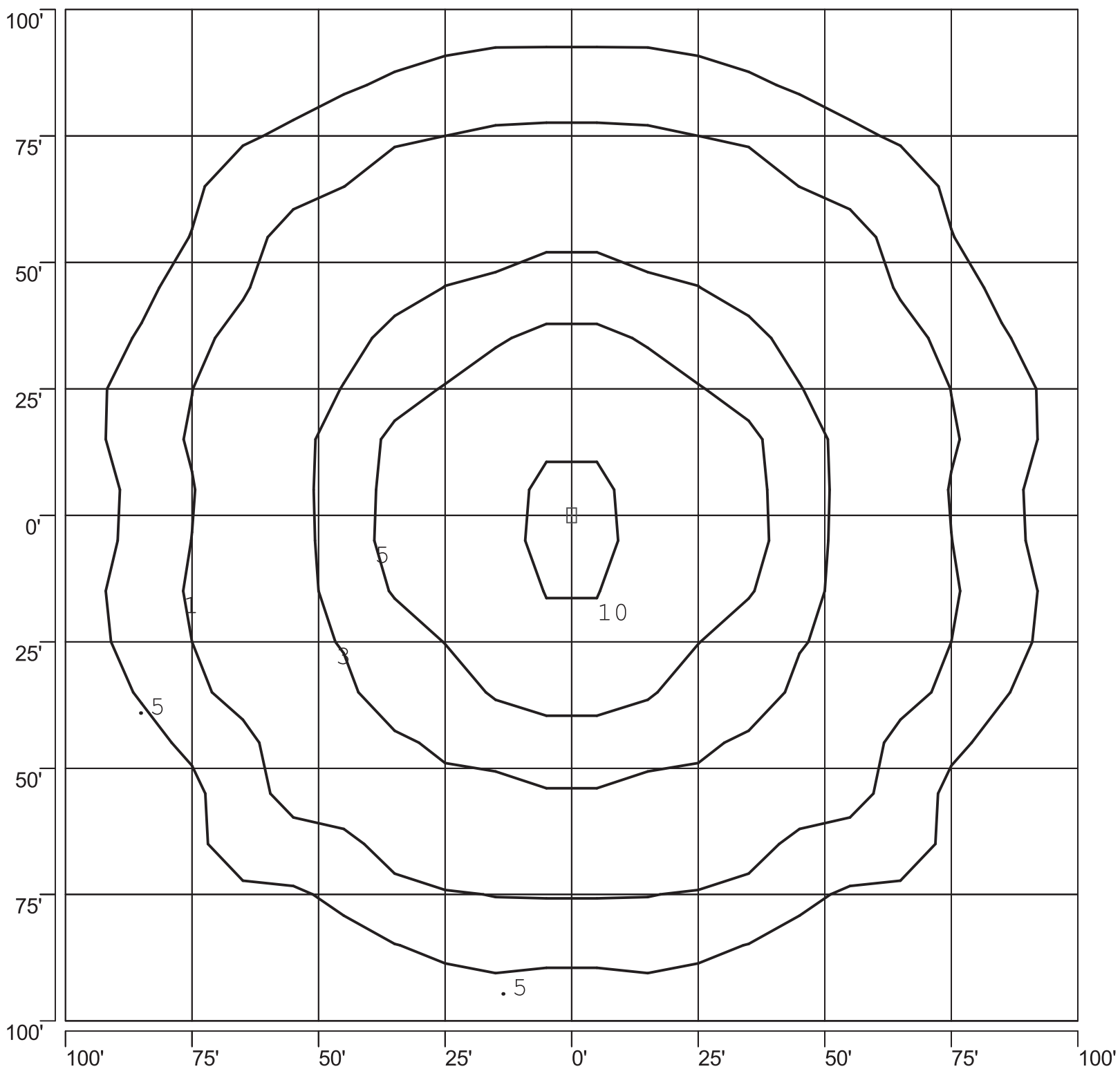
ISOFOOTCANDLE PLOT: VBLAF1B_1 1000W MH TYPE V 30' AFG - 0 DEGREE TILT
