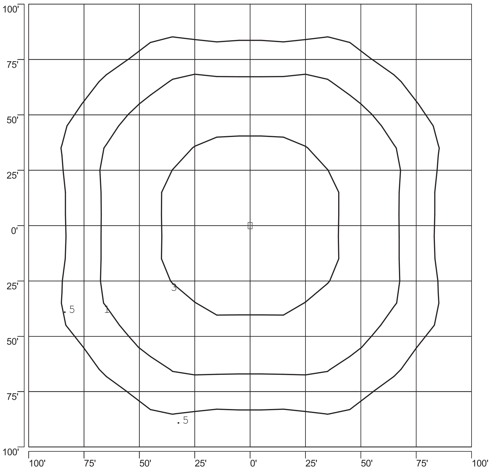
ISOFOOTCANDLE PLOT: VBLAE6B_2-PS 750W PSMH TYPE V 30' AFG - 0 DEGREE TILT
