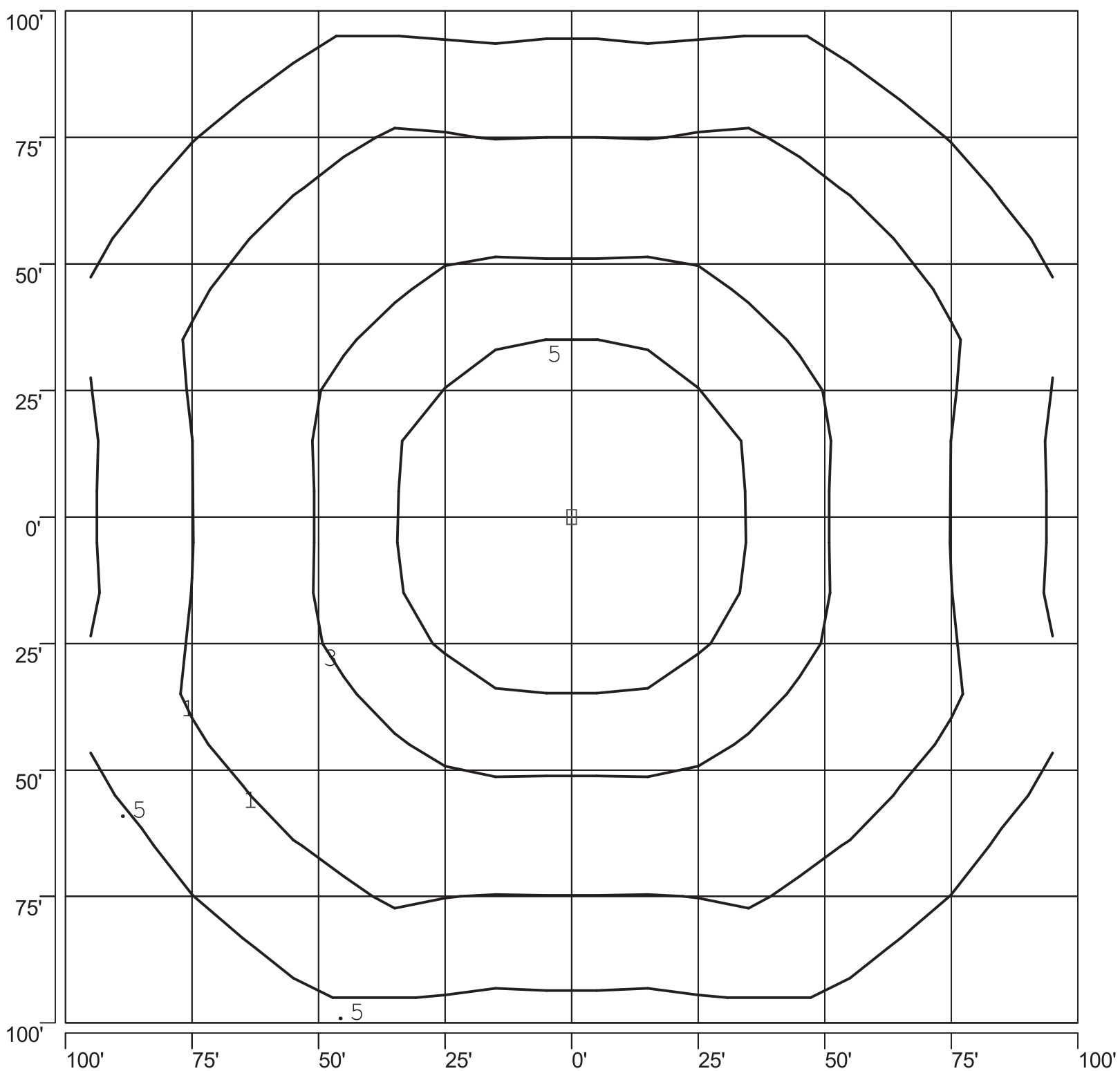
ISOFOOTCANDLE PLOT: VBLAE1B_2 1000W MH TYPE V 30' AFG - 0 DEGREE TILT
