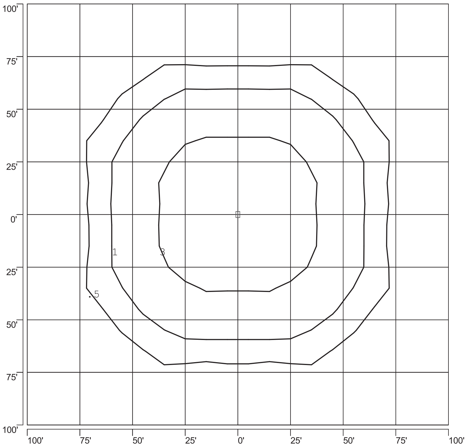
ISOFOOTCANDLE PLOT: VBLAC6B_2-PS 750W PSMH TYPE V 30' AFG - 0 DEGREE TILT
