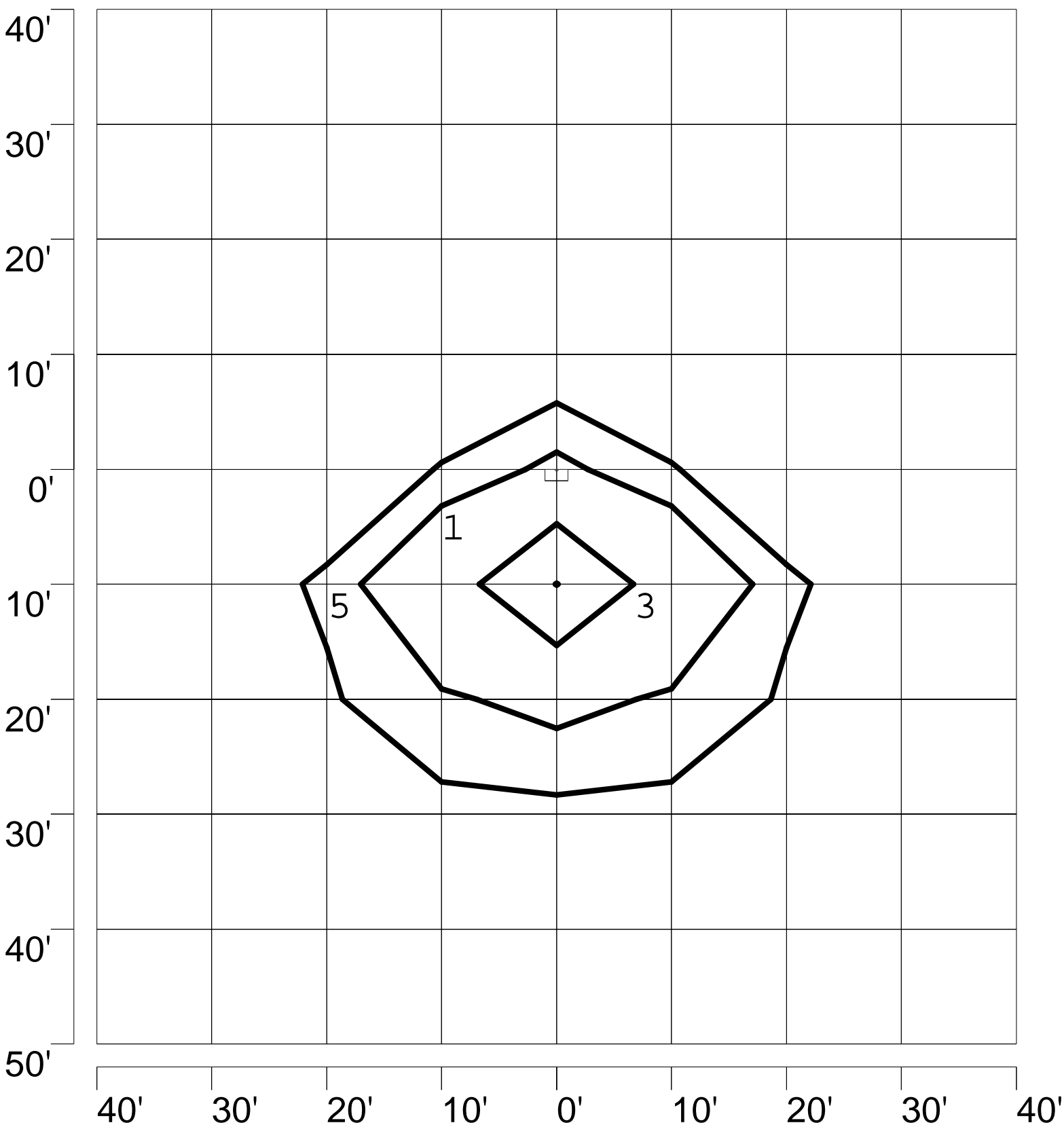
ISOFOOTCANDLE PLOT: RWPB2A-OPEN CLR ROUND WALL PACK 8' AFG - 0 DEGREE TILT
