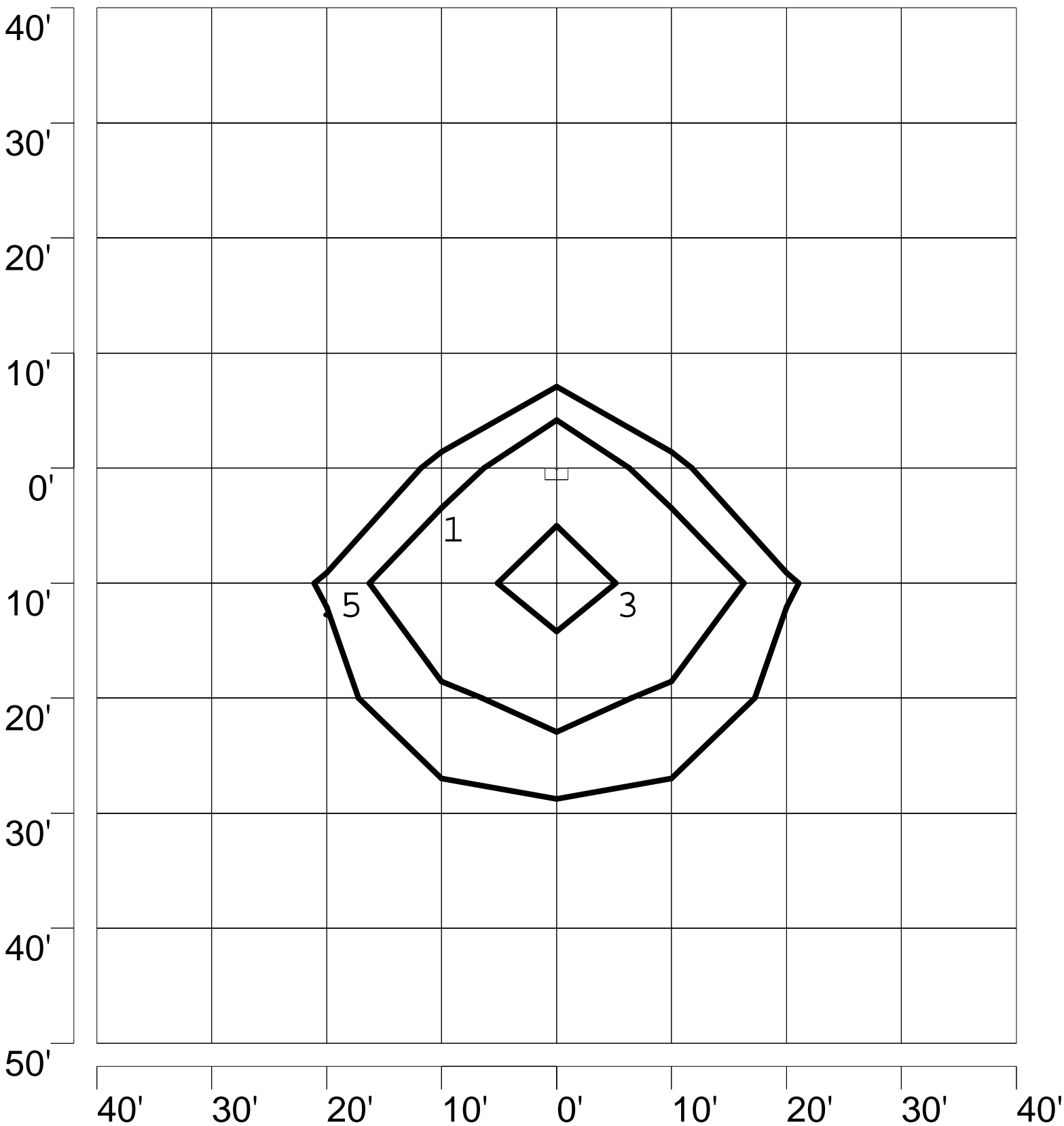
ISOFOOTCANDLE PLOT: RWPB2A-TOP CUTOFF CLR ROUND WALL PACK 8' AFG - 0 DEGREE TILT
