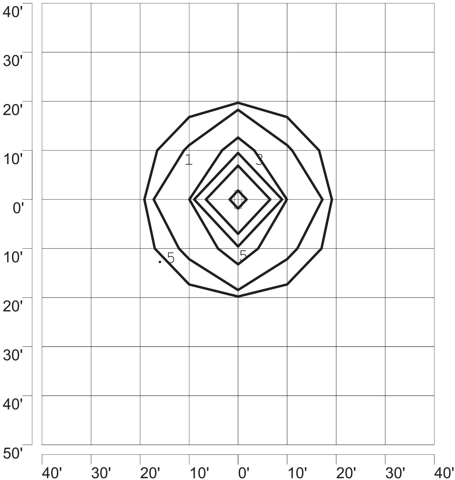
ISOFOOTCANDLE PLOT: RCLSRF1A DUAL LAMP FLUOR REC CANOPY 10' AFG - 0 DEGREE TILT
