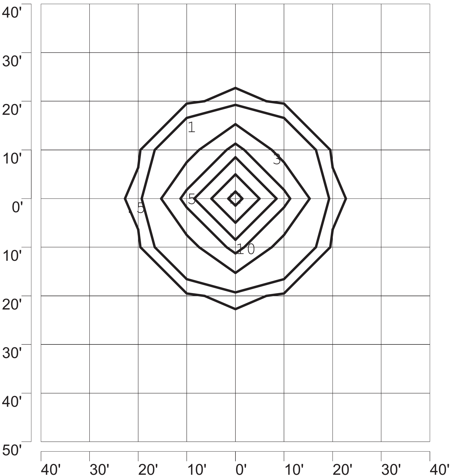
ISOFOOTCANDLE PLOT: RCLS21 150W PSMH RECESSED CANOPY 10' AFG - 0 DEGREE TILT
