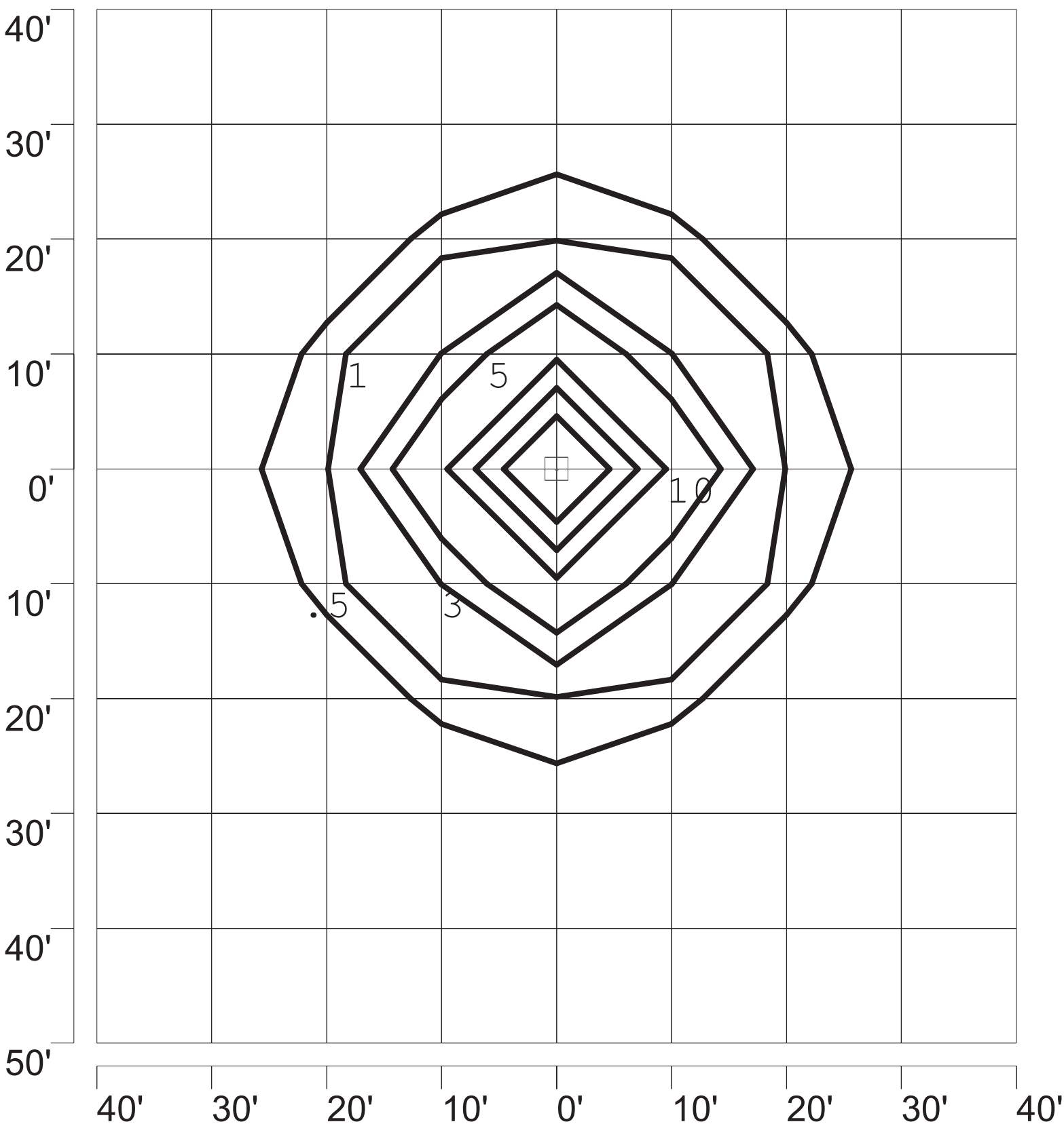
ISOFOOTCANDLE PLOT: RCLS07 250W PSMH RECESSED CANOPY 10' AFG - 0 DEGREE TILT
