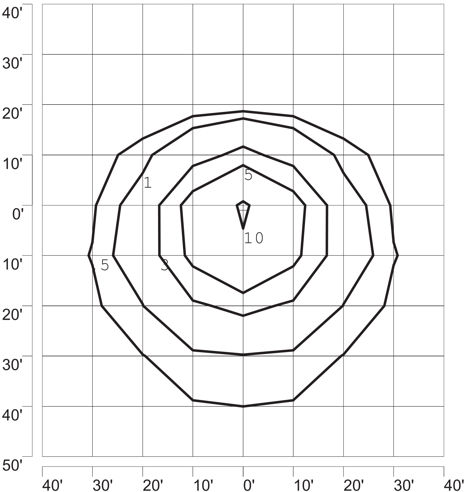
ISOFOOTCANDLE PLOT: MWPF9A-CO-150W PSMH FT CO WALL PACK 15' AFG - 0 DEGREE TILT
