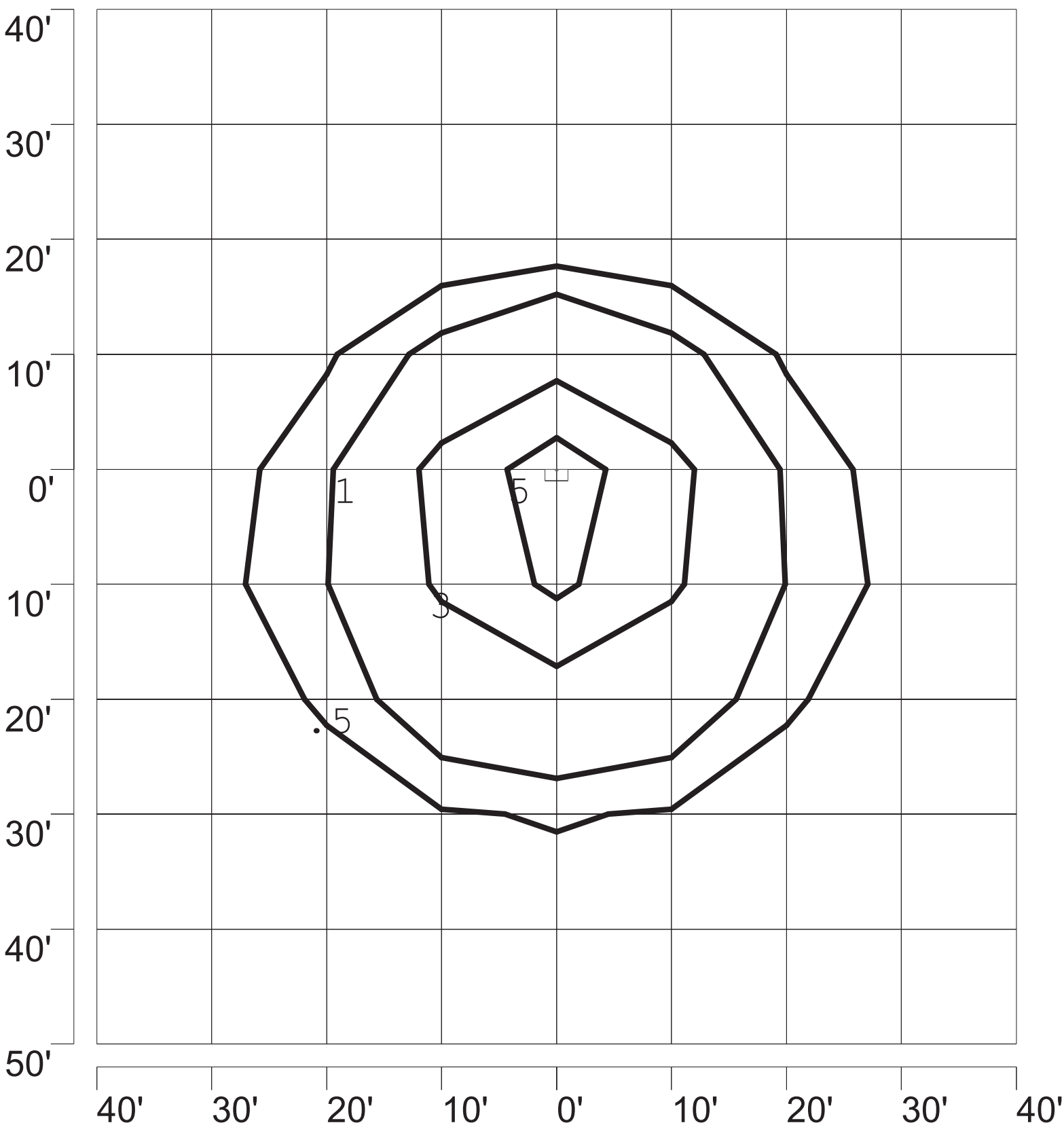
ISOFOOTCANDLE PLOT: MWPF2A-CO-100W MH FT CO WALL PACK 15' AFG - 0 DEGREE TILT
