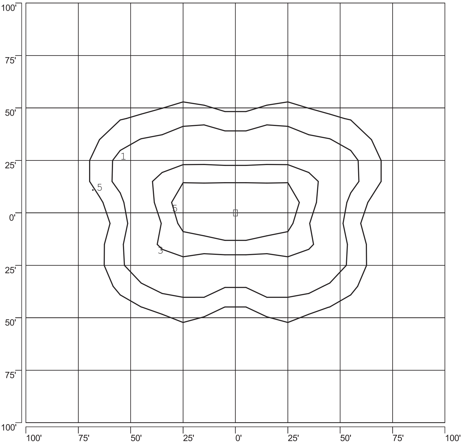
ISOFOOTCANDLE PLOT: MSBBE3A_-PS 400W PSMH TYPE V 25' AFG - 0 DEGREE TILT
