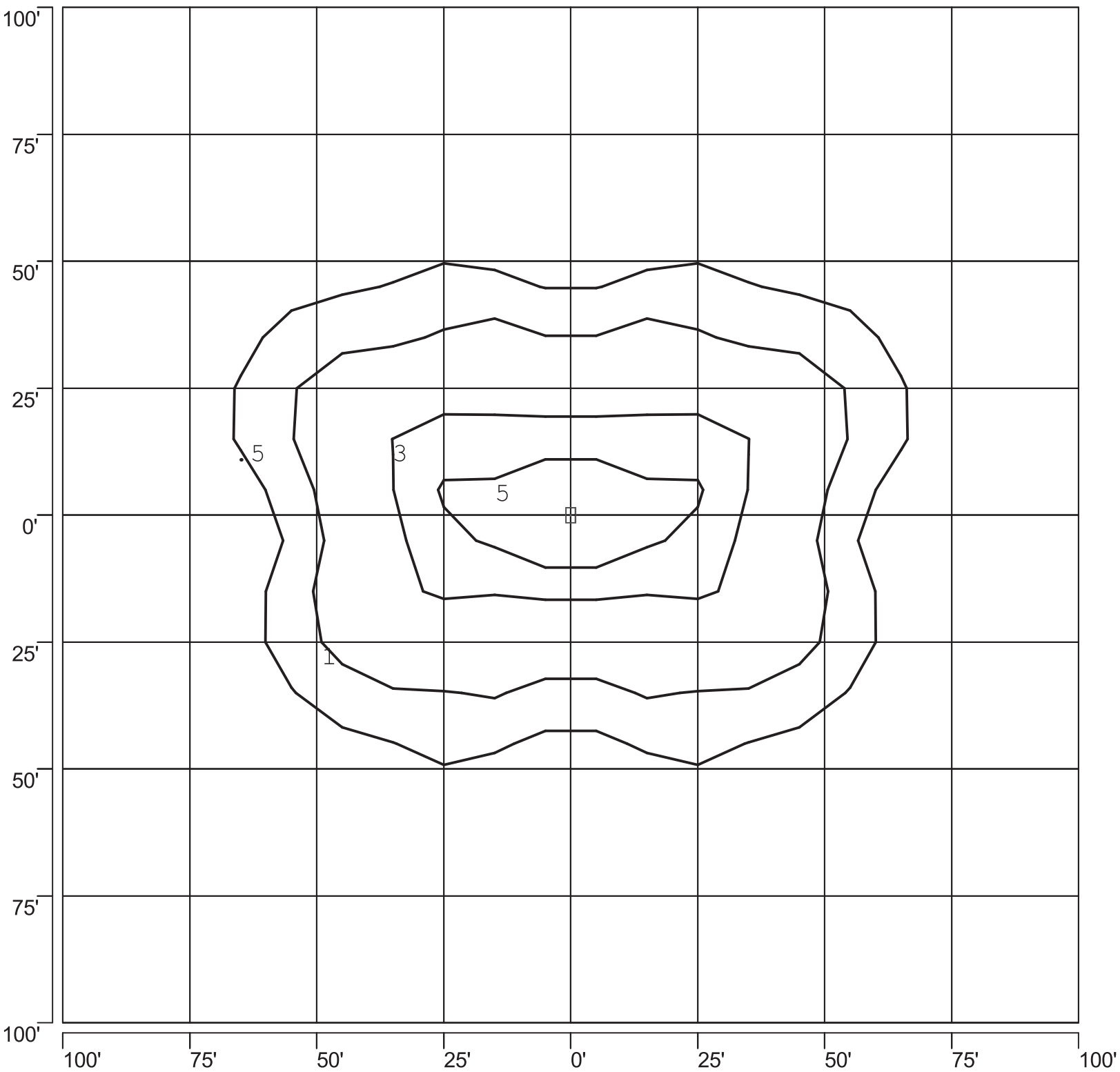
ISOFOOTCANDLE PLOT: MSBBE2A_-PS 250W PSMH TYPE V 25' AFG - 0 DEGREE TILT
