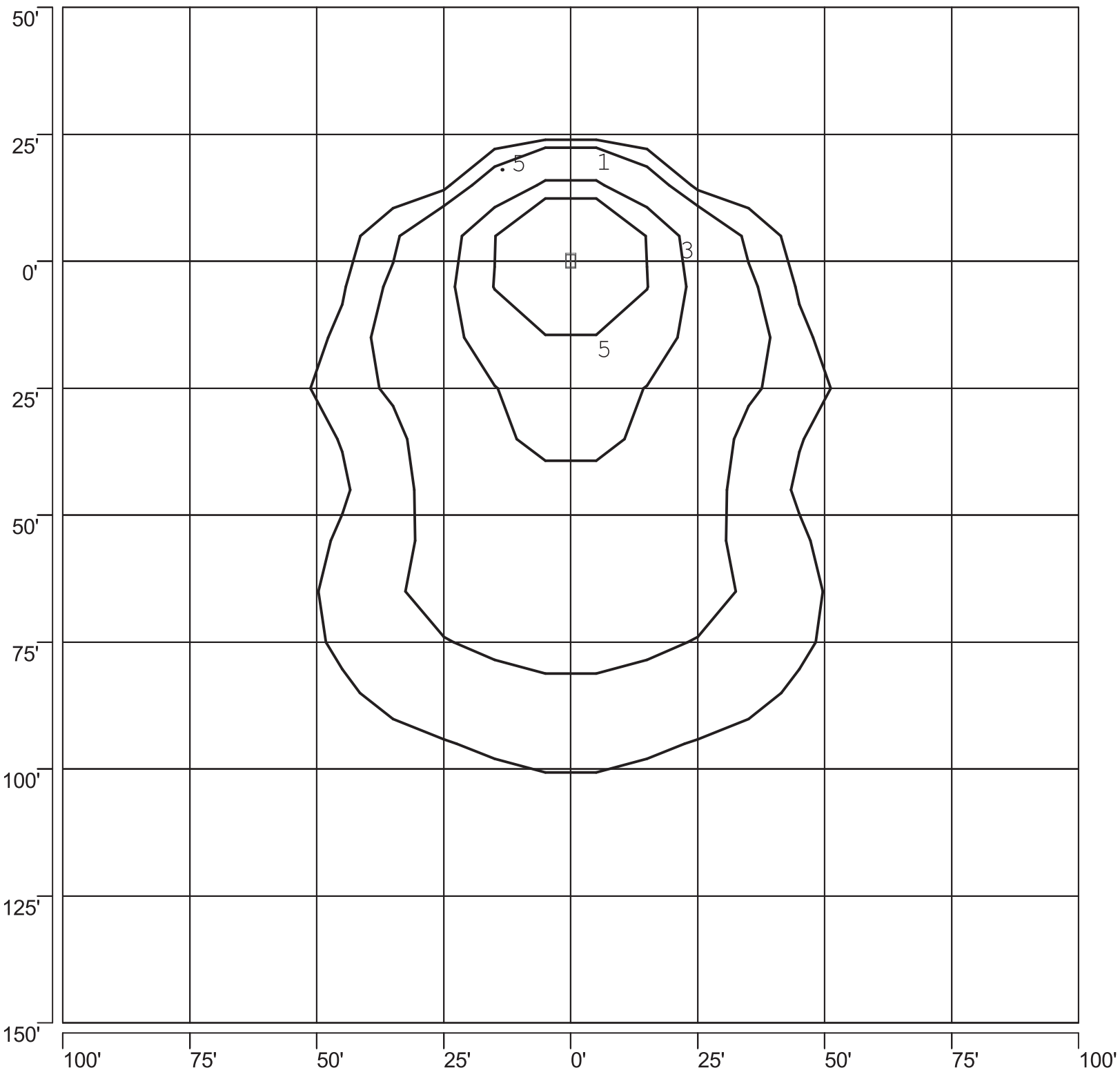
ISOFOOTCANDLE PLOT: MSBBD3A_-PS 400W PSMH CUTOFF FLOOD 25' AFG - 25 DEGREE TILT
