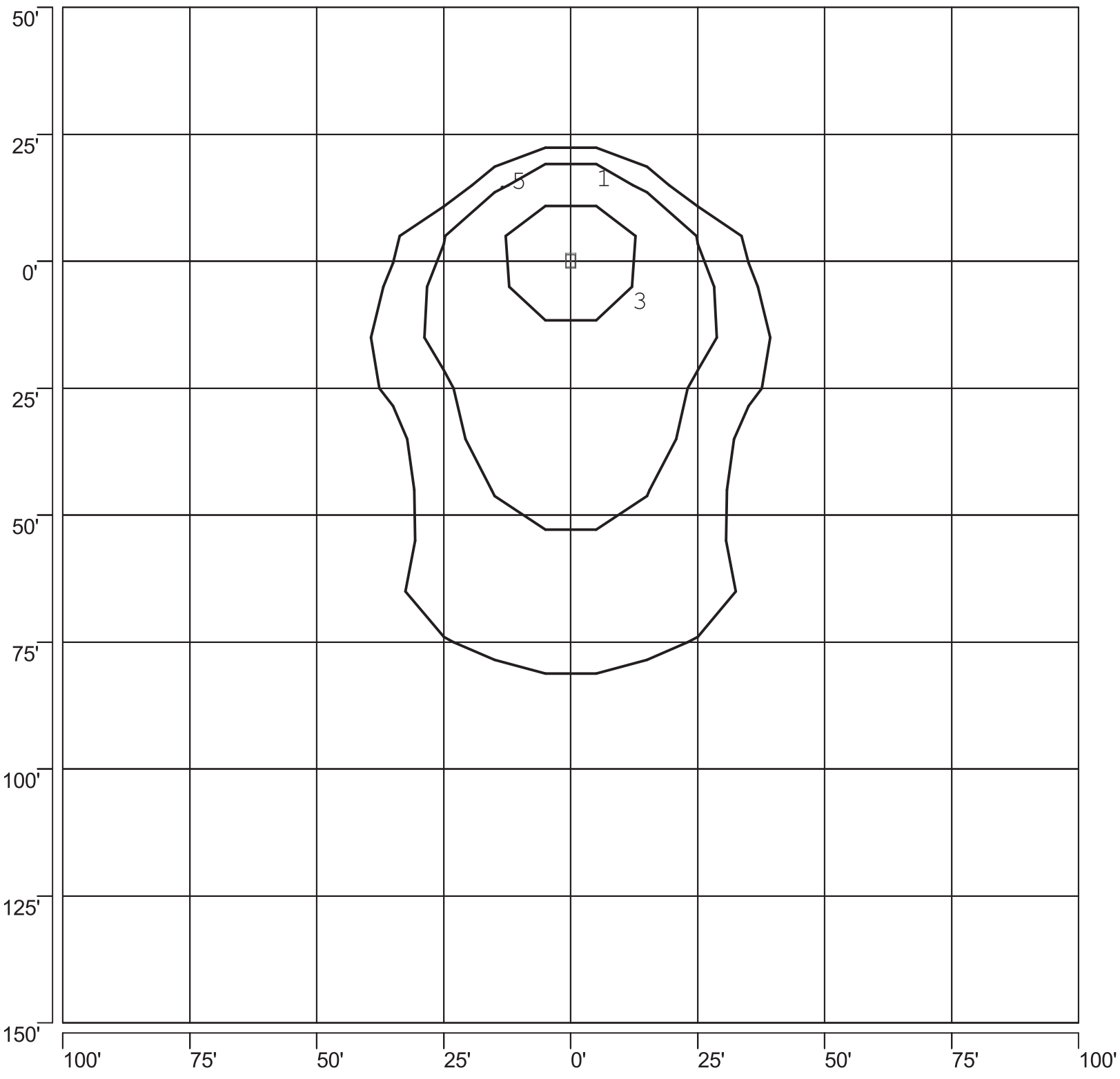
ISOFOOTCANDLE PLOT: MSBBD2A_-PS 250W PSMH CUTOFF FLOOD 25' AFG - 25 DEGREE TILT
