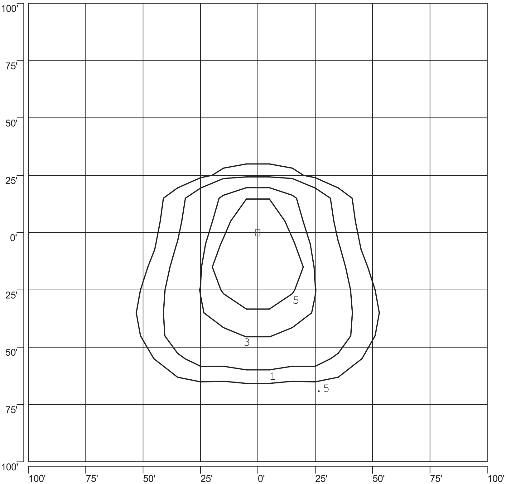
ISOFOOTCANDLE PLOT: MSBBB3A_-PS 400W PSMH TYPE IV 25' AFG - 0 DEGREE TILT
