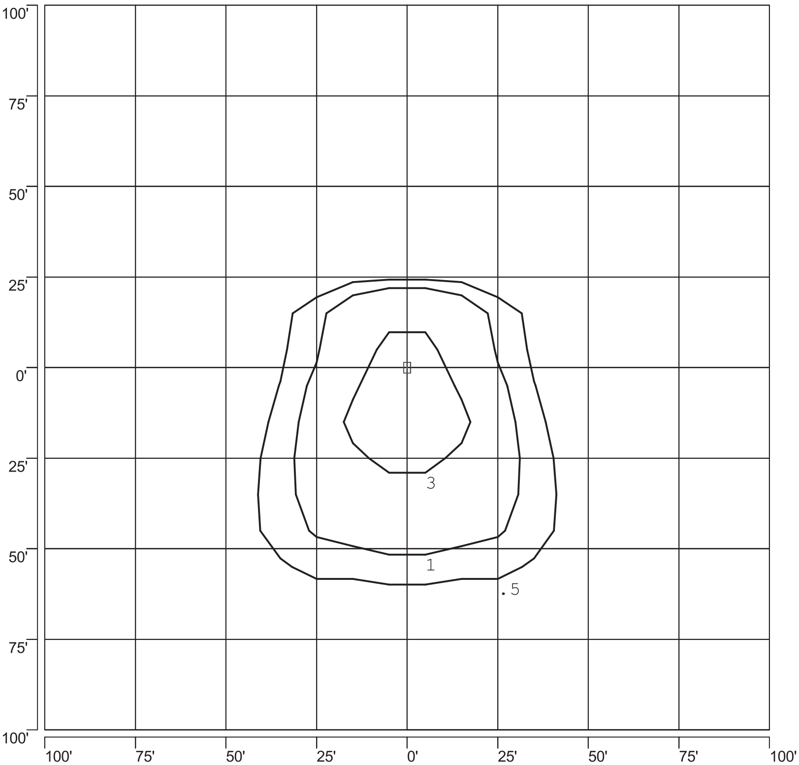
ISOFOOTCANDLE PLOT: MSBBB2A_-PS 250W PSMH TYPE IV 25' AFG - 0 DEGREE TILT
