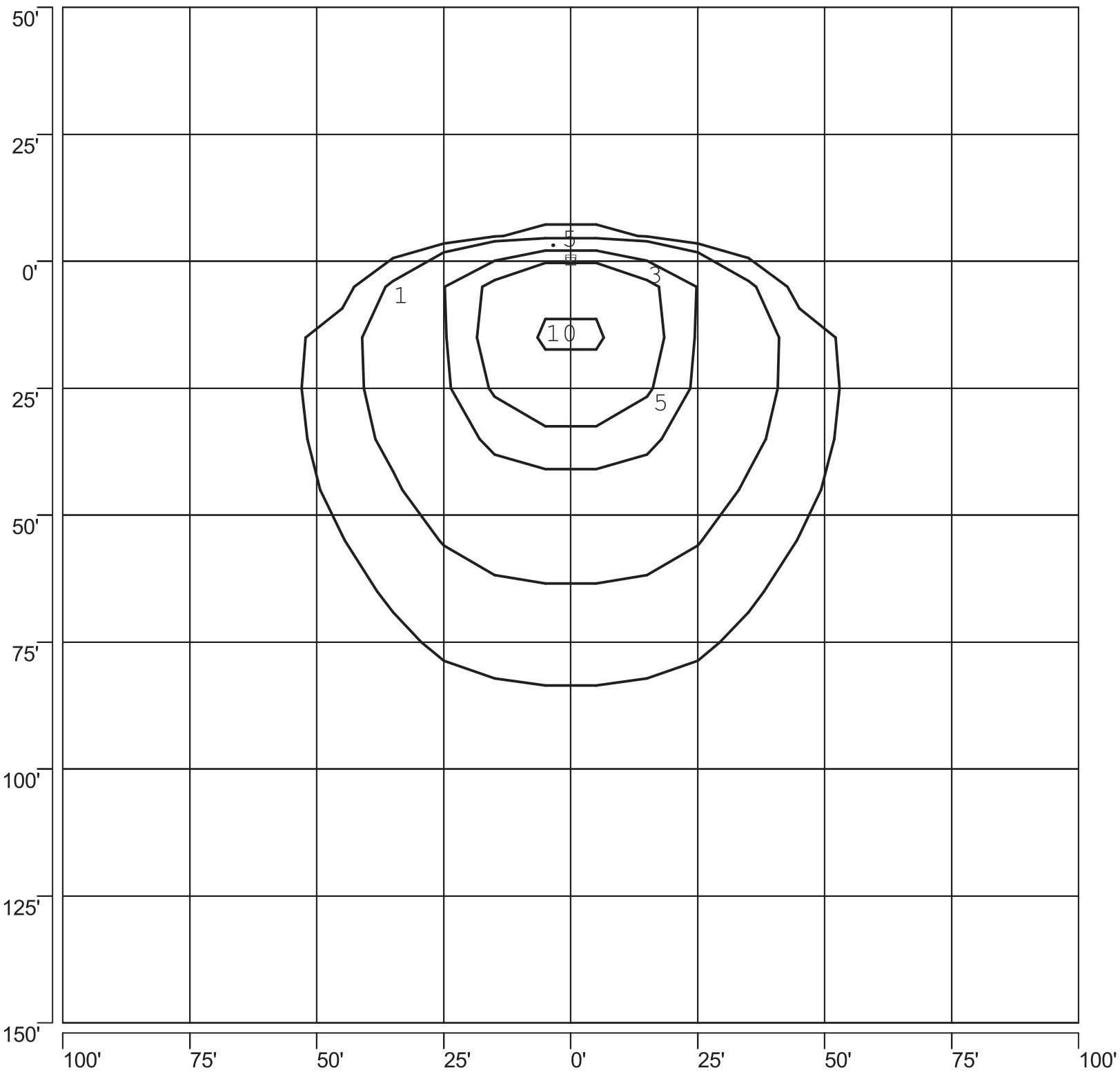
ISOFOOTCANDLE PLOT: MSBBA3A_-PS 400W PSMH STANDARD FLOOD 25' AFG - 60 DEGREE TILT
