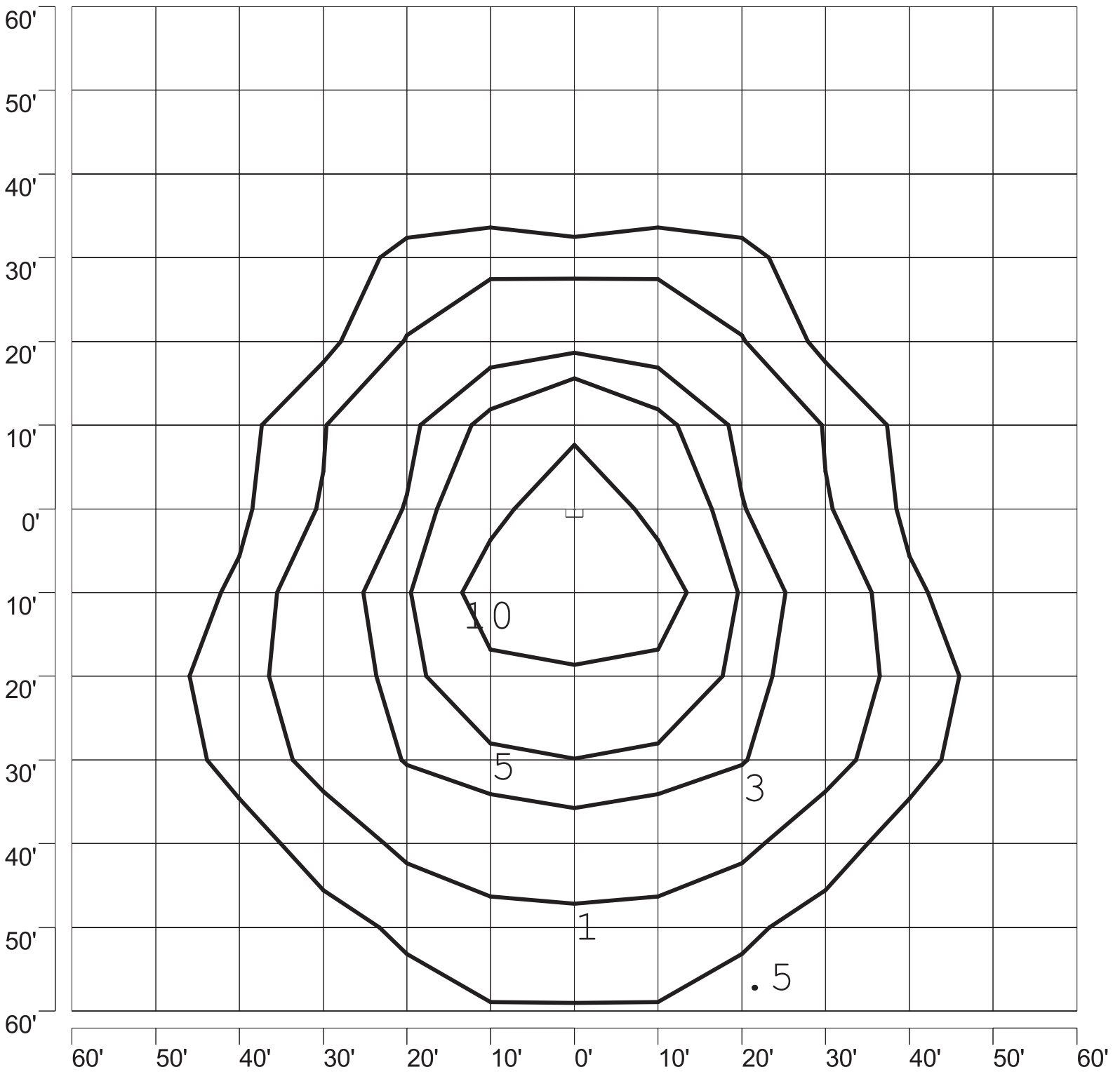
ISOFOOTCANDLE PLOT: LWPF4A-PS-CO-400W PSMH FT CO WALL PACK 20' AFG - 0 DEGREE TILT
