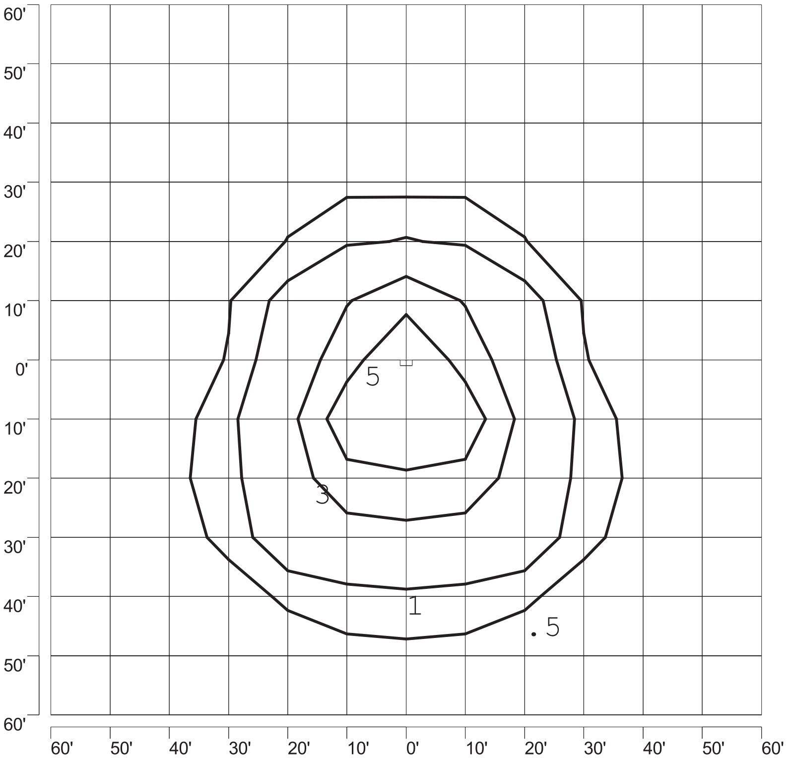
ISOFOOTCANDLE PLOT: LWPF2A-PS-CO-250W PSMH FT CO WALL PACK 20' AFG - 0 DEGREE TILT
