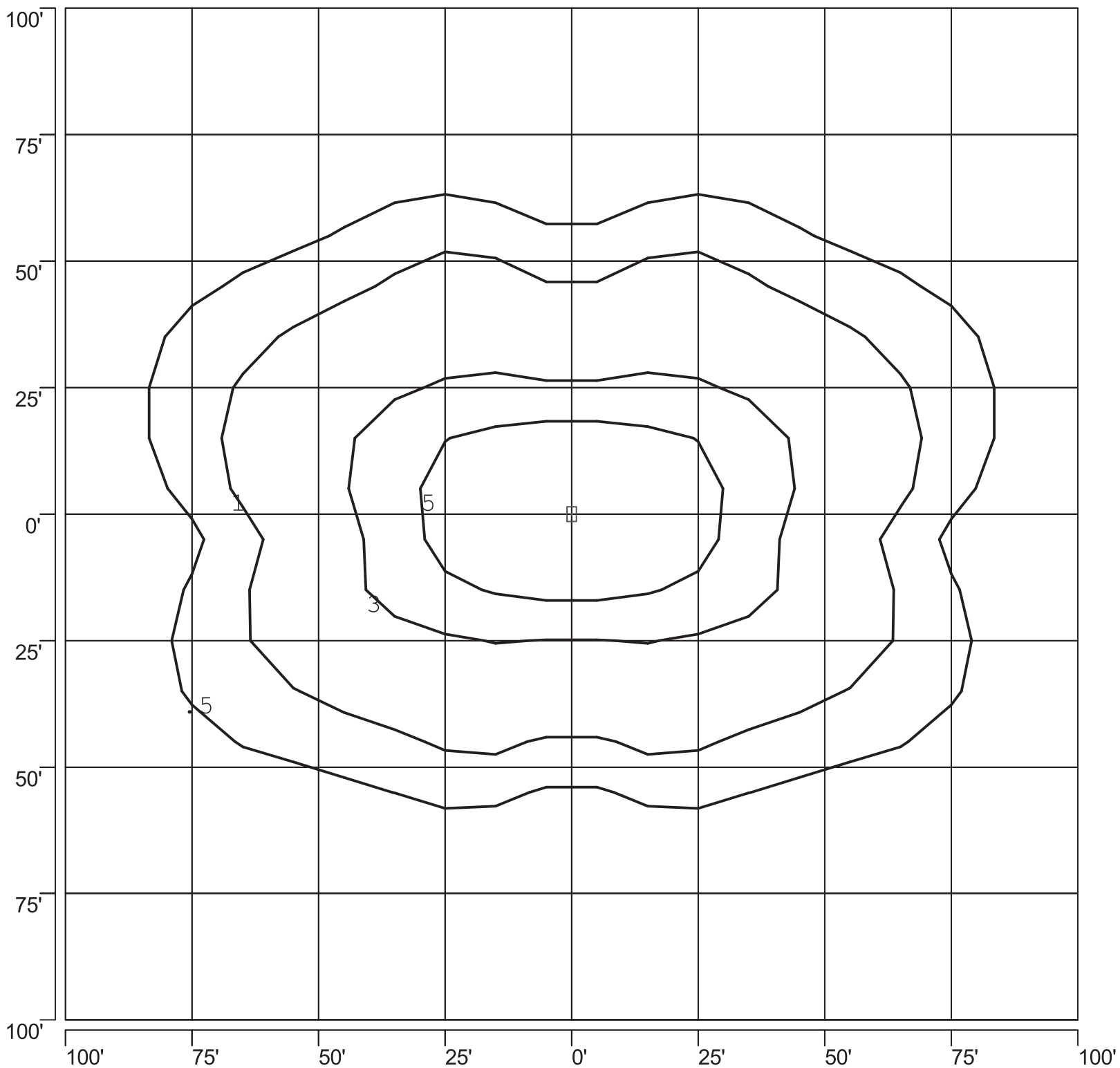
ISOFOOTCANDLE PLOT: LSBBE11_1-PS-750W PSMH TYPE V 30' AFG - 0 DEGREE TILT
