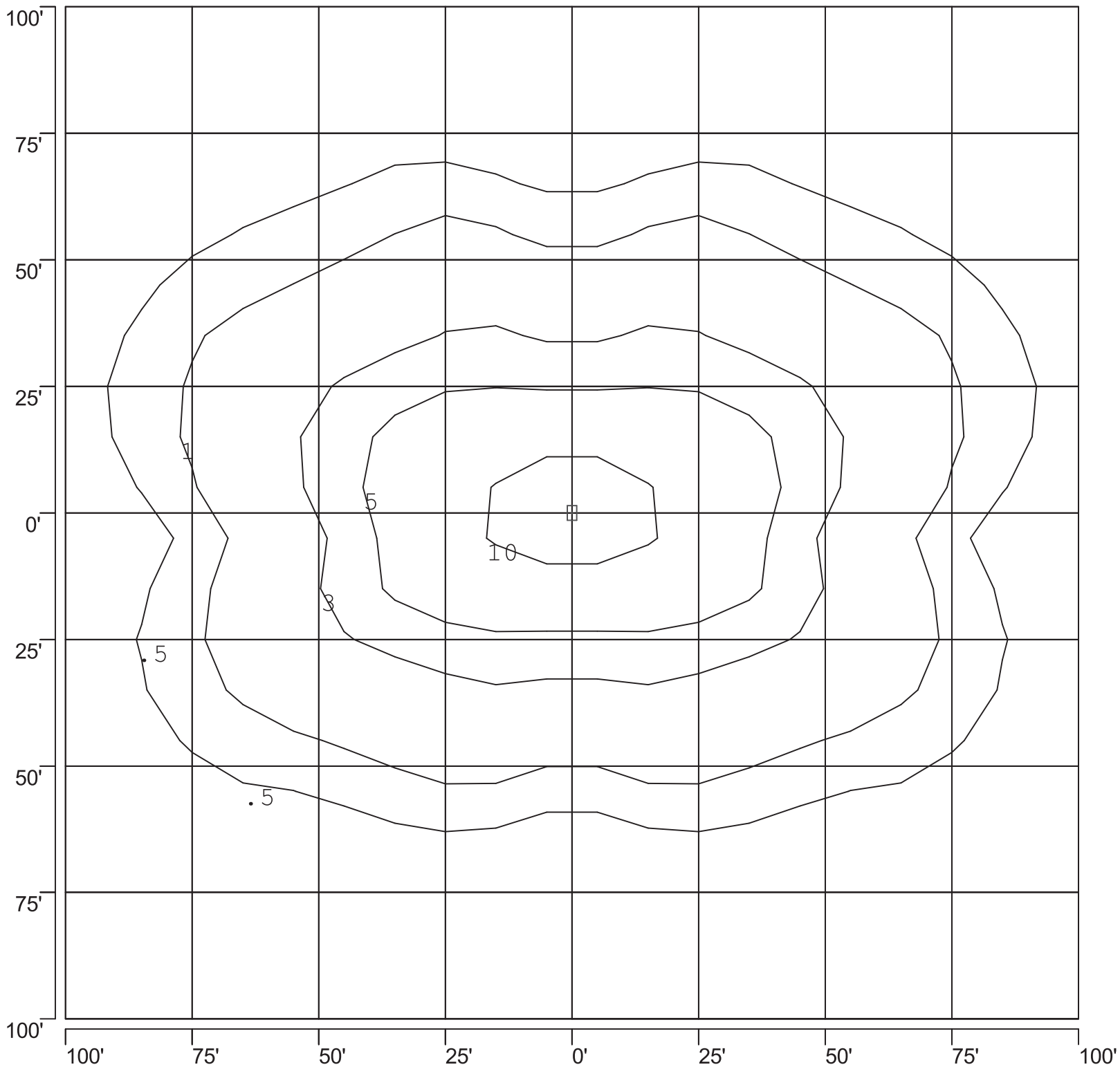
ISOFOOTCANDLE PLOT: LSBBE1_1-1000W MH TYPE V 30' AFG - 0 DEGREE TILT
