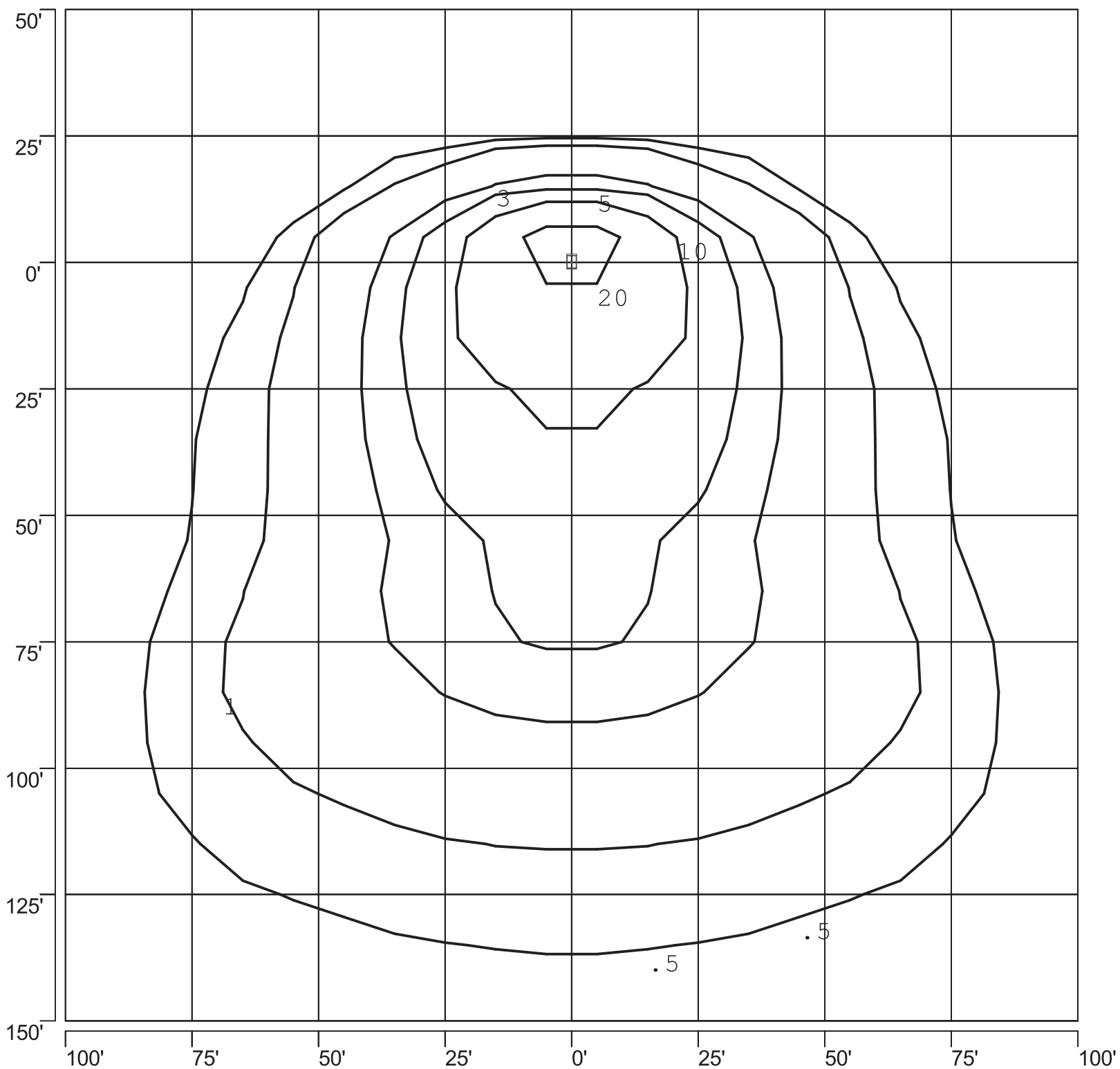
ISOFOOTCANDLE PLOT: LSBBD2A1-1000W HPS CUTOFF FLOOD 30' AFG - 25 DEGREE TILT
