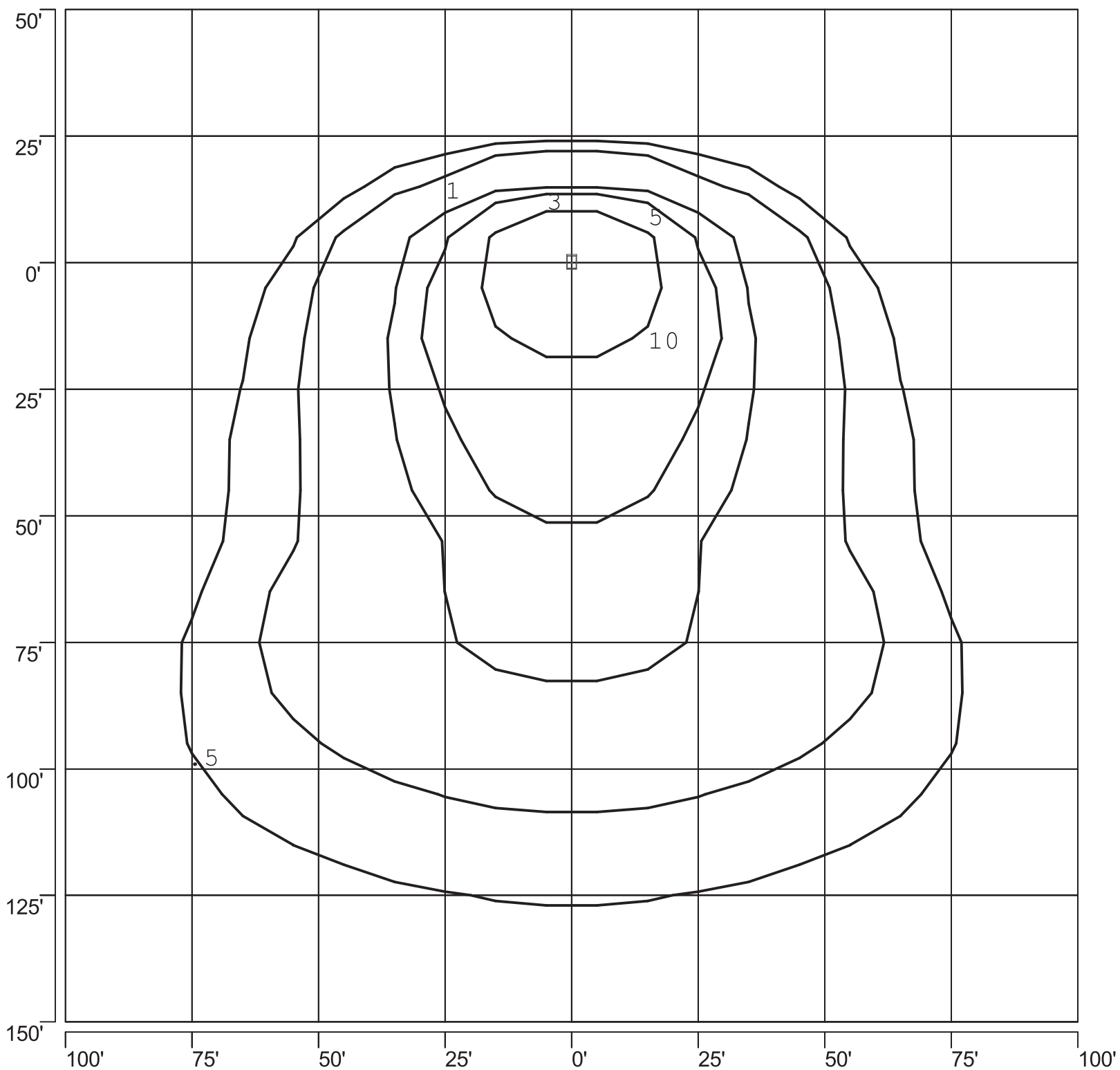
ISOFOOTCANDLE PLOT: LSBBD1_1-1000W MH CUTOFF FLOOD 30' AFG - 25 DEGREE TILT
