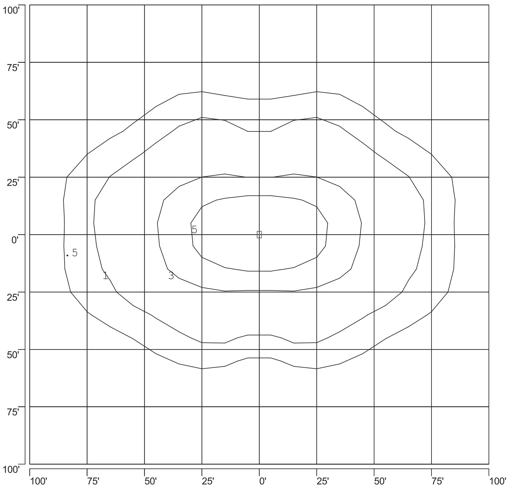
ISOFOOTCANDLE PLOT: LSBBC11_1-PS-750W PSMH TYPE II 30' AFG - 0 DEGREE TILT
