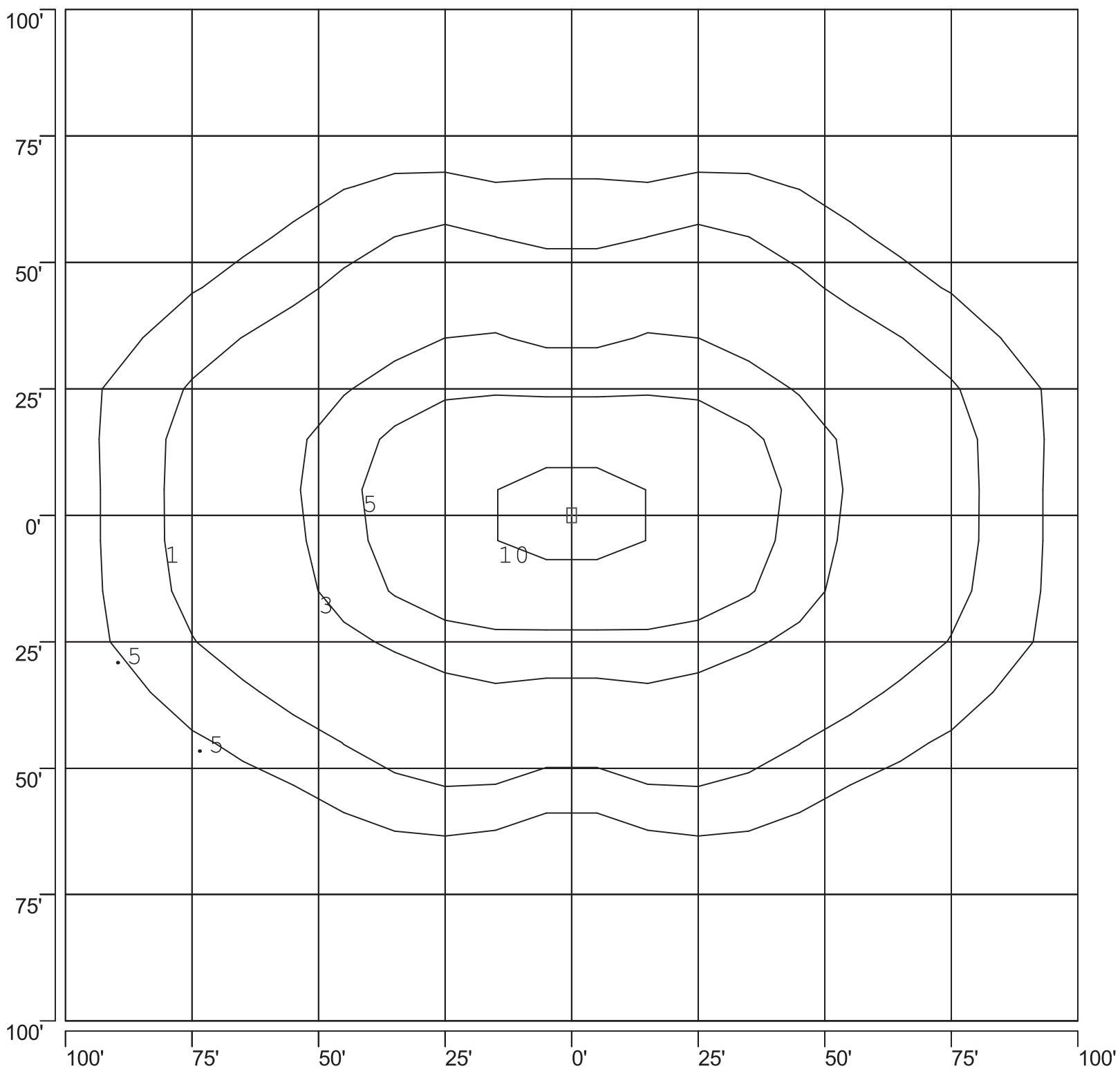
ISOFOOTCANDLE PLOT: LSBBC1_1-1000W MH TYPE II 30' AFG - 0 DEGREE TILT
