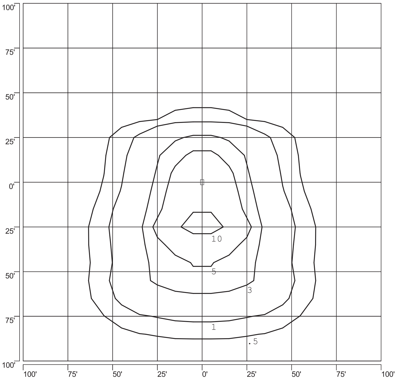
ISOFOOTCANDLE PLOT: LSBBB11_1-PS-750W PSMH TYPE IV 30' AFG - 0 DEGREE TILT
