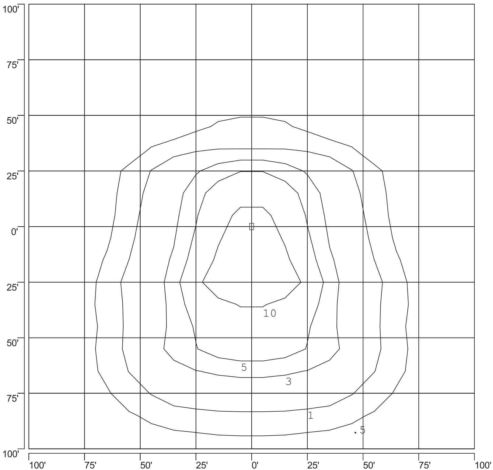
ISOFOOTCANDLE PLOT: LSBBB1_1-1000W MH TYPE IV 30' AFG - 0 DEGREE TILT
