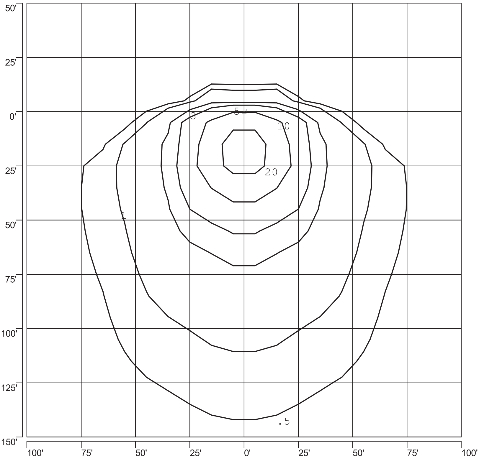
ISOFOOTCANDLE PLOT: LSBBA2A1-1000W HPS STANDARD FLOOD 30' AFG - 60 DEGREE TILT
