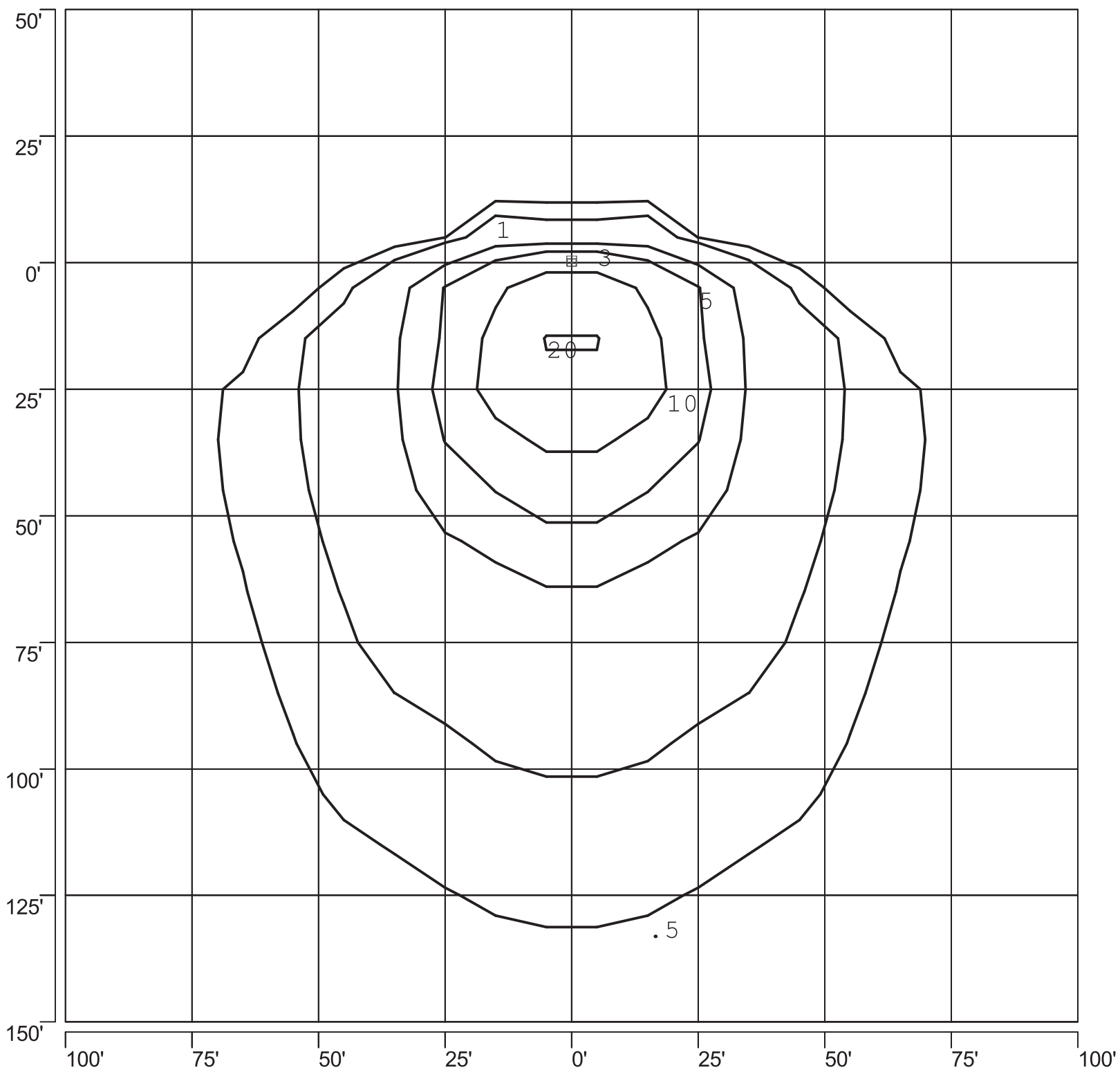
ISOFOOTCANDLE PLOT: LSBBA1_1-1000W MH STANDARD FLOOD 30' AFG - 60 DEGREE TILT
