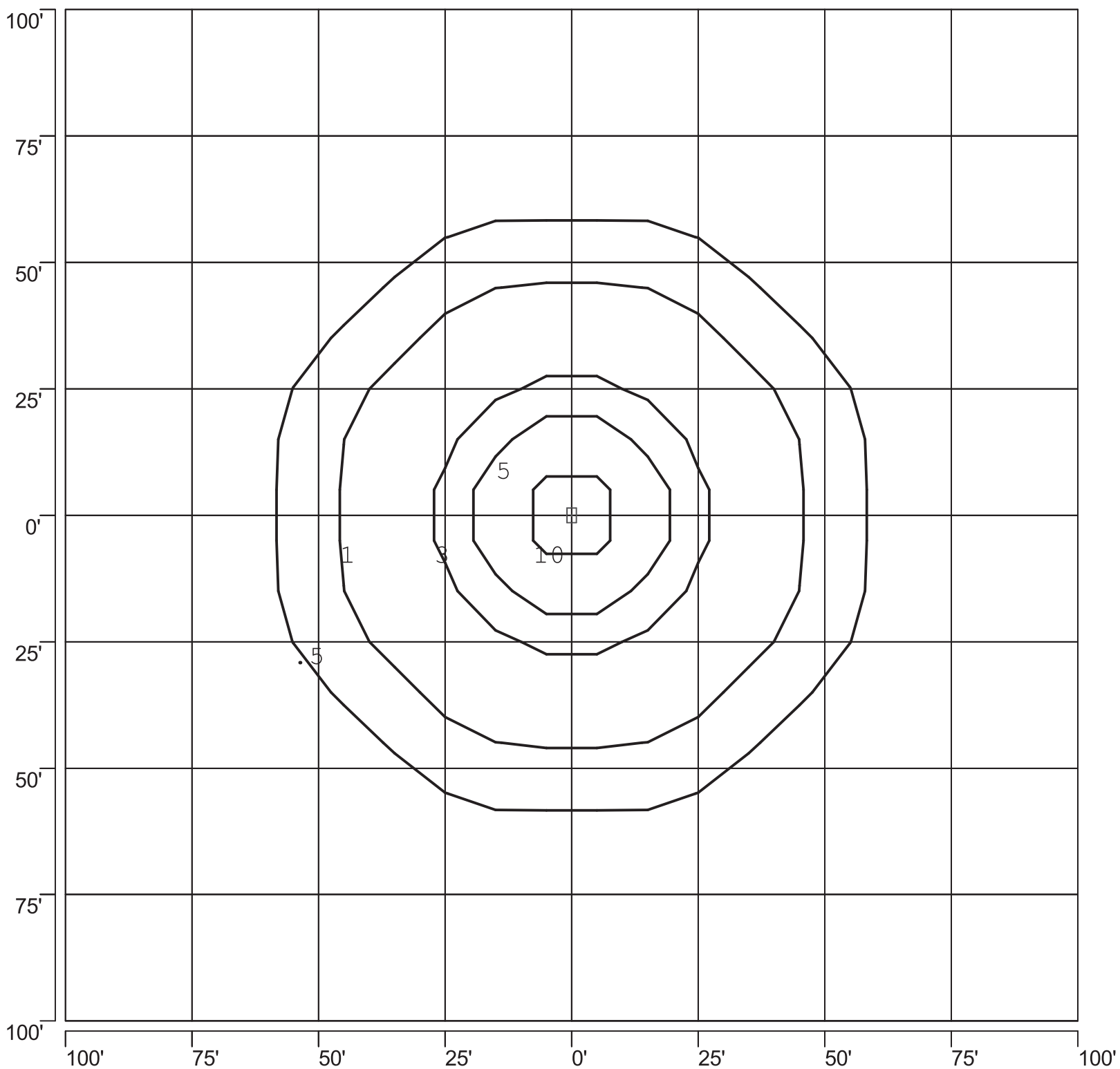
ISOFOOTCANDLE PLOT: ENT-51-403-277-402-2 400W PSMH TYPE V VERT 25' AFG - 0 DEGREE TILT
