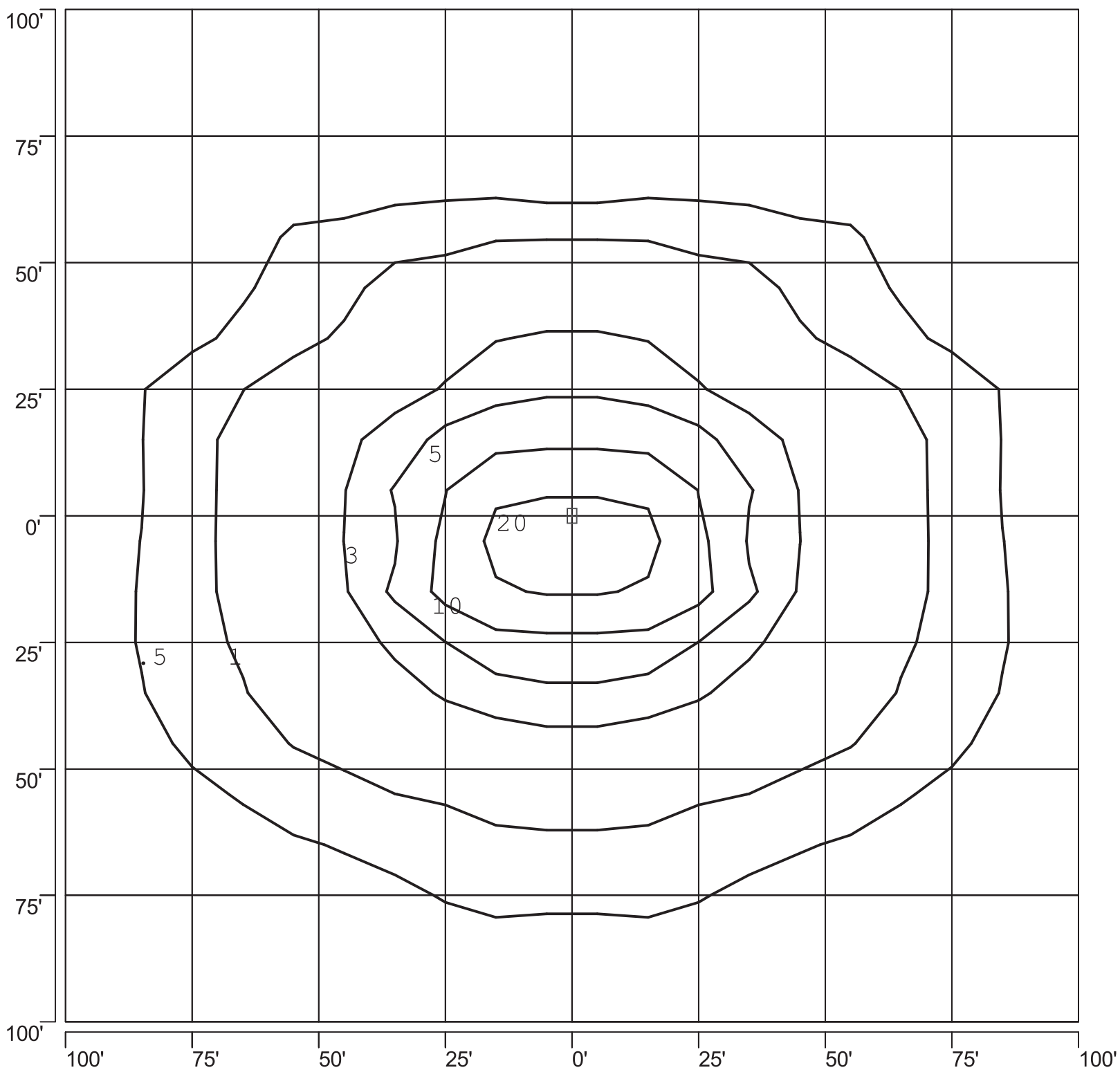
ISOFOOTCANDLE PLOT: ENT-44-900-277-900-2 1000W MH TYPE IV VERT 30' AFG - 0 DEGREE TILT
