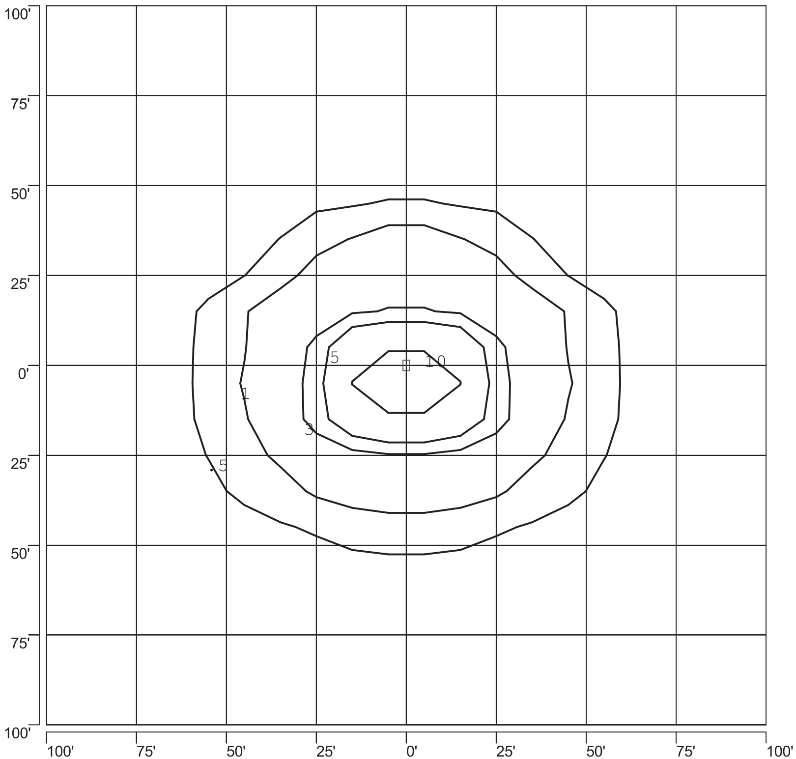
ISOFOOTCANDLE PLOT: ENT-44-403-277-402-2 4000W PSMH TYPE IV VERT 25' AFG - 0 DEGREE TILT
