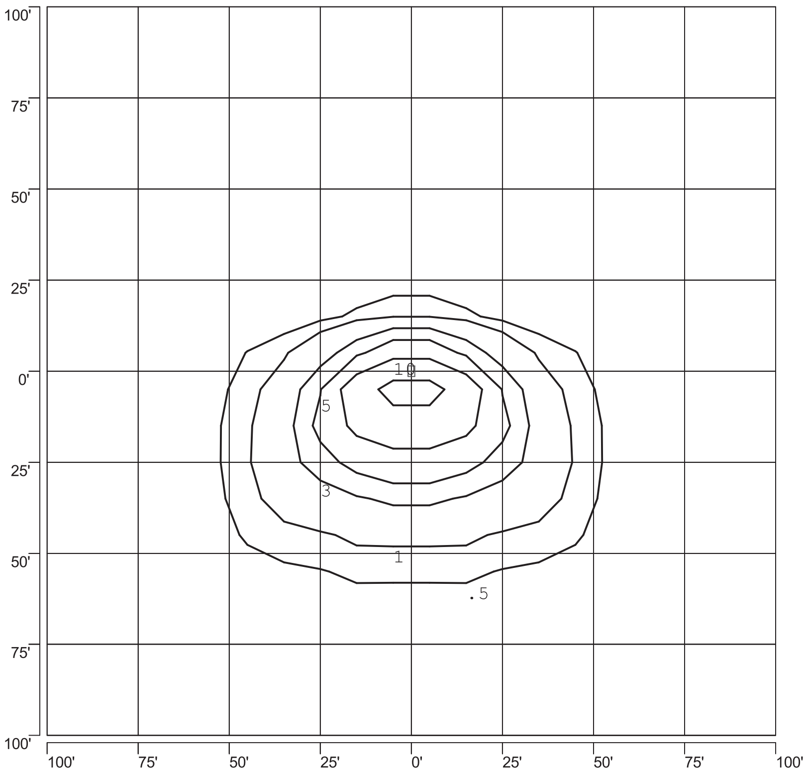
ISOFOOTCANDLE PLOT: ENT-43-403-277-402-1 400W PSMH TYPE IV AUTO 25' AFG - 0 DEGREE TILT
