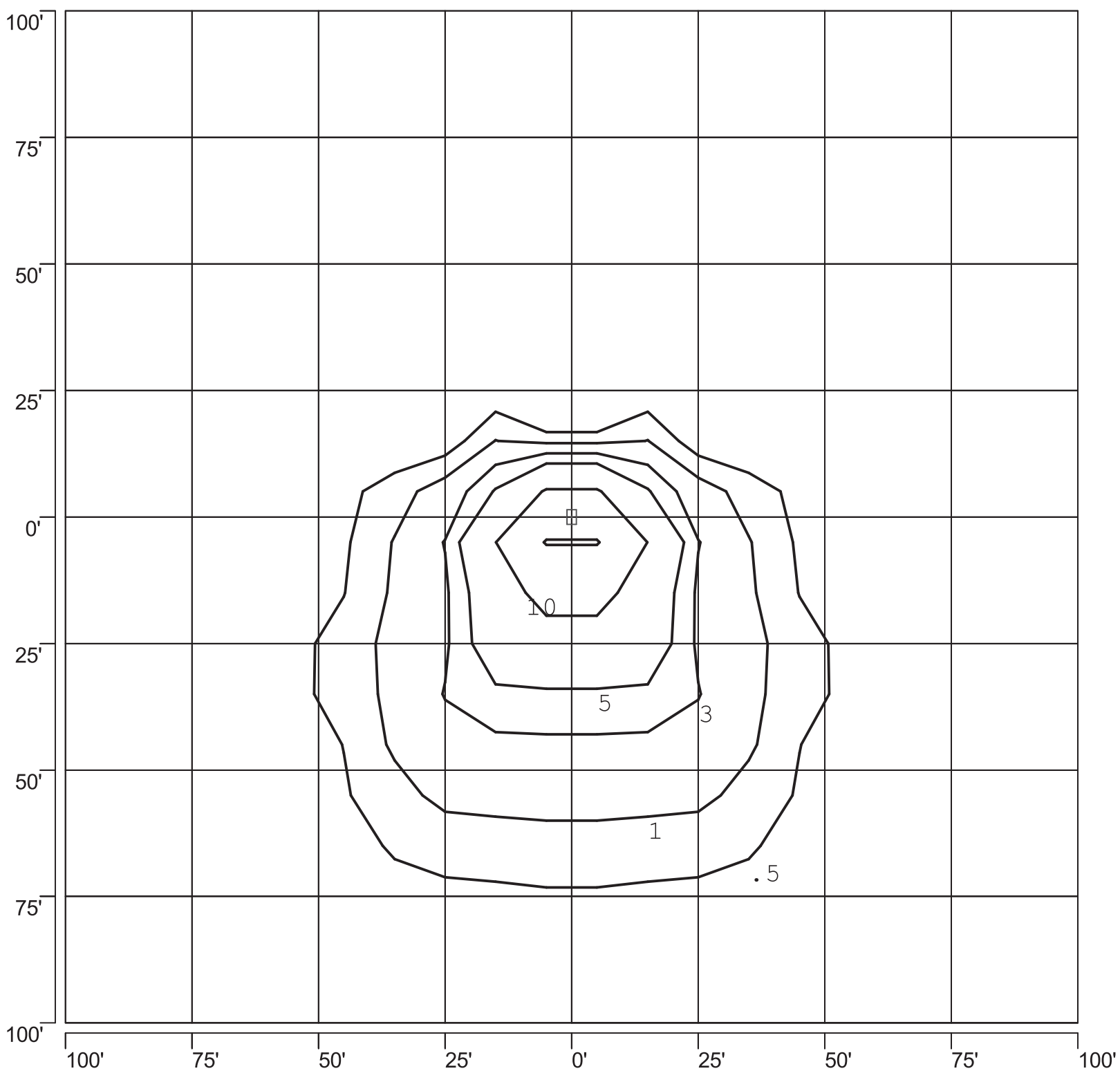
ISOFOOTCANDLE PLOT: ENT-40-403-277-402-1 400W PSMH TYPE IV HOR 25' AFG - 0 DEGREE TILT
