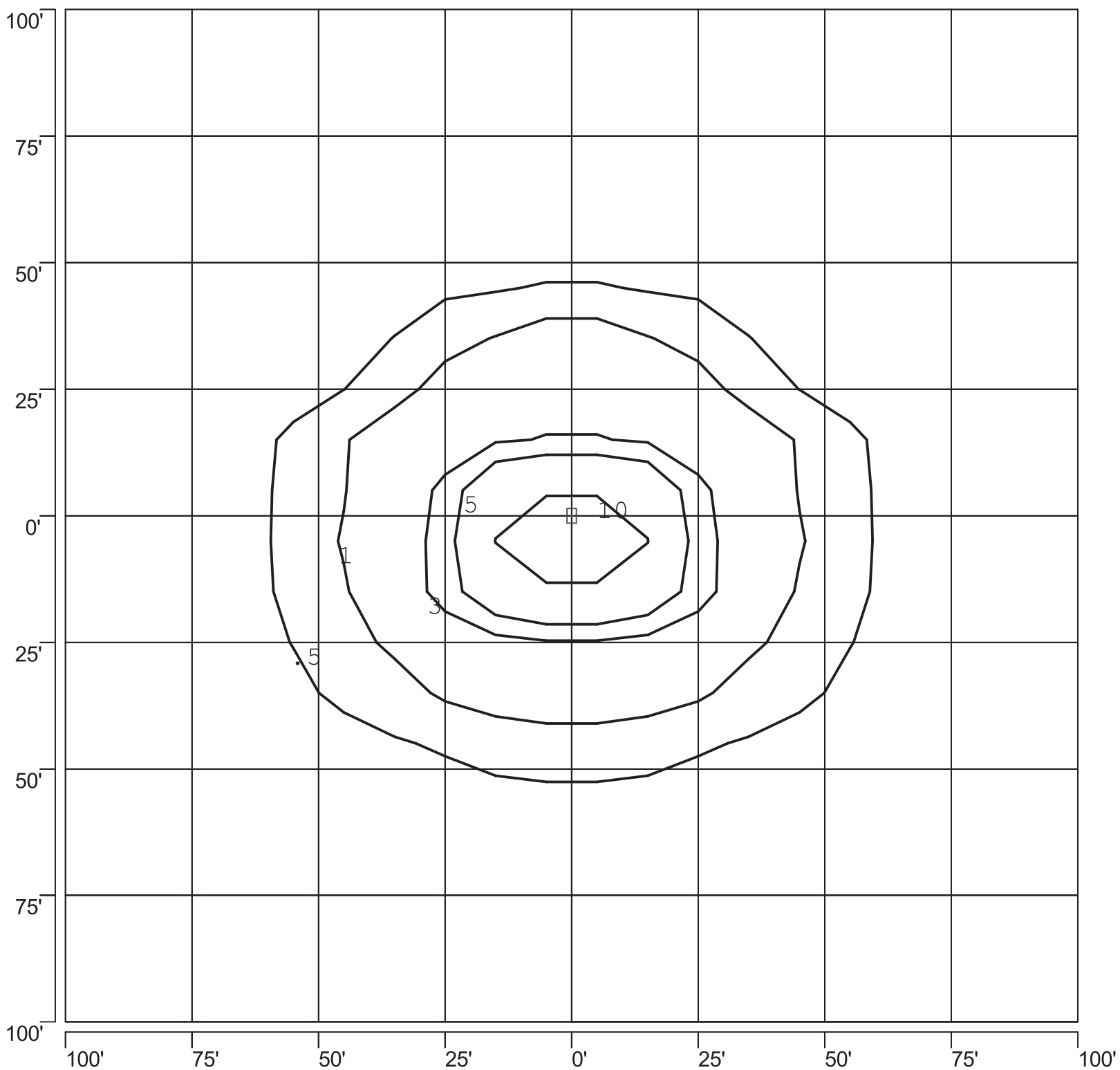
ISOFOOTCANDLE PLOT: ENT-31-403-277-402-2 400W PSMH TYPE III VERT 25' AFG - 0 DEGREE TILT
