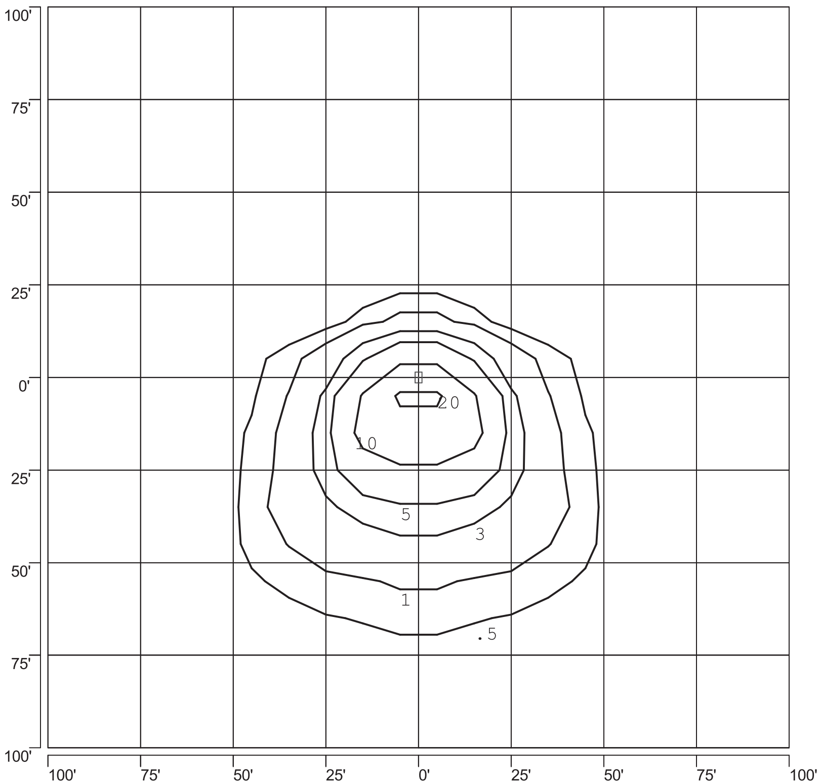
ISOFOOTCANDLE PLOT: ENT-30-403-277-402-1 400W PSMH TYPE III HOR 25' AFG - 0 DEGREE TILT
