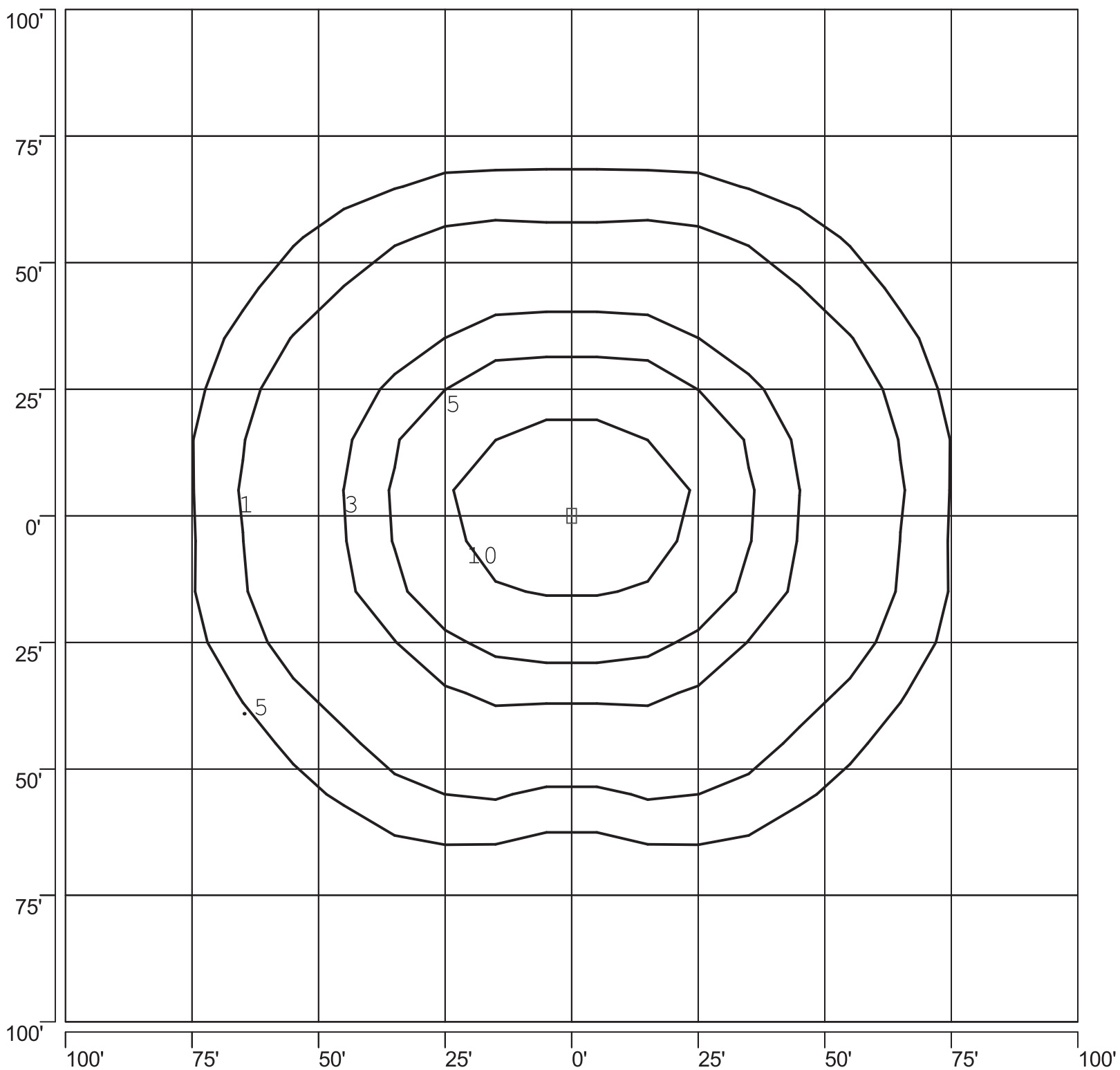
ISOFOOTCANDLE PLOT: ENT-20-900-277-900-1 1000W MH TYPE II HOR 30' AFG - 0 DEGREE TILT
