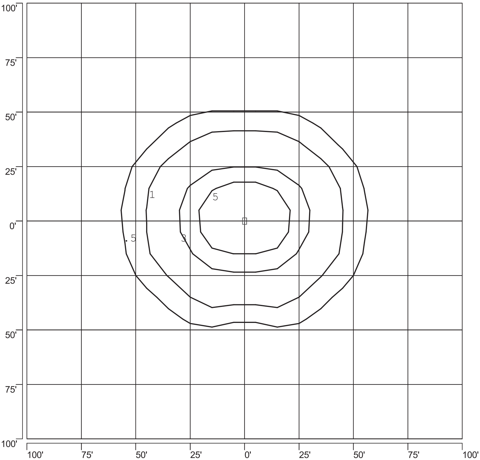
ISOFOOTCANDLE PLOT: ENT-20-403-277-402-1 400W PSMH TYPE II HOR 25' AFG - 0 DEGREE TILT
